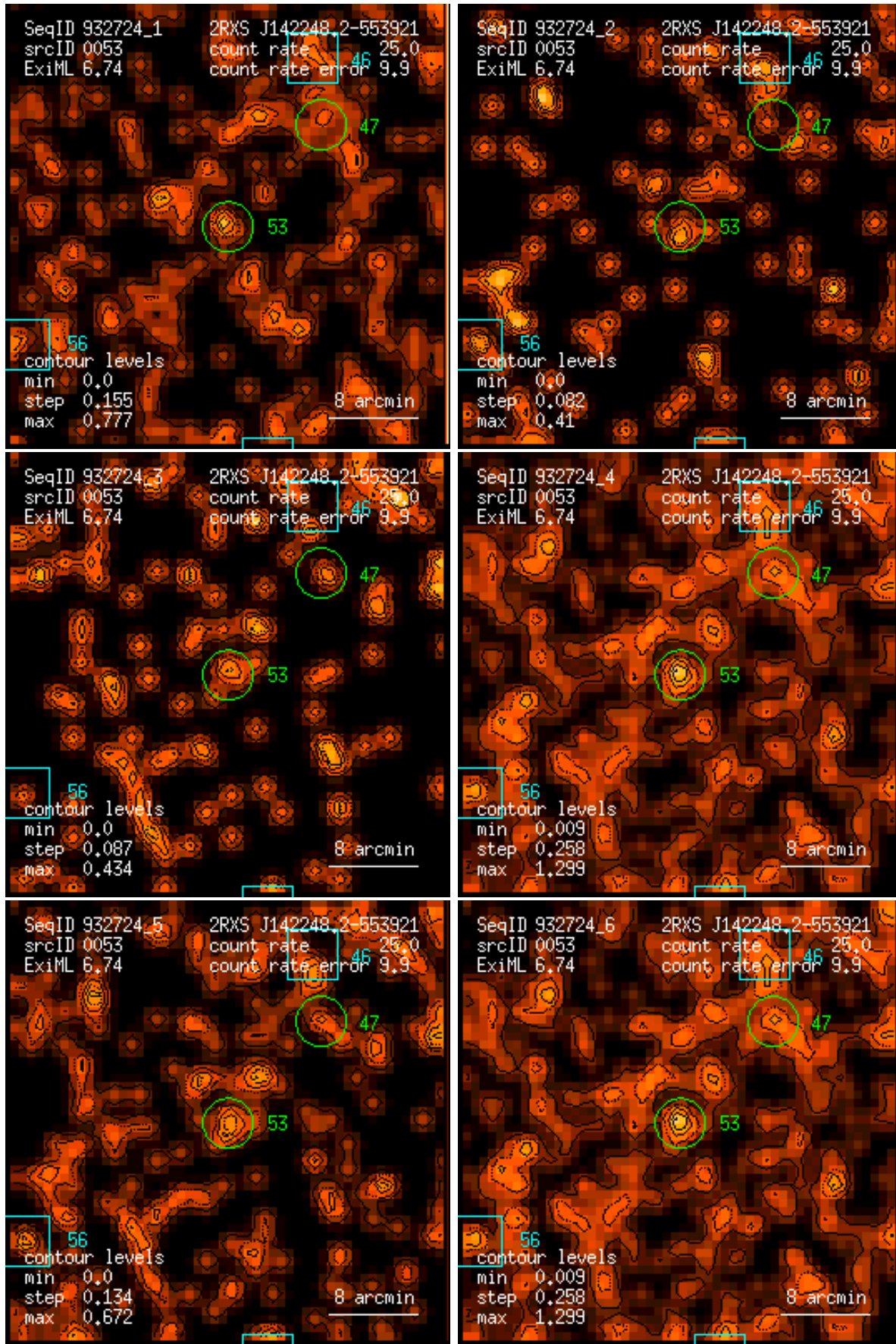
Figure 53: RASS 932724: detection 0053: band rate images, Gaussian filter: (1) PSPC channels 11 – 41, (2) 52 – 90, (3) 91 – 201, (4) 11 – 235, (5) 52 – 201, (6) 11 – 201. Broad band rates in counts/ks. Band rate contour levels in counts/ks/arcmin 2 .
