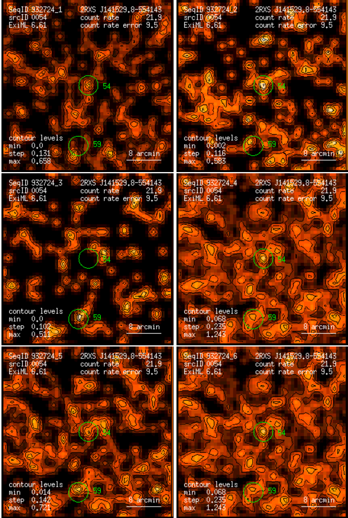
Figure 54: RASS 932724: detection 0054: band rate images, Gaussian filter: (1) PSPC channels 11 – 41, (2) 52 – 90, (3) 91 – 201, (4) 11 – 235, (5) 52 – 201, (6) 11 – 201. Broad band rates in counts/ks. Band rate contour levels in counts/ks/arcmin 2 .
