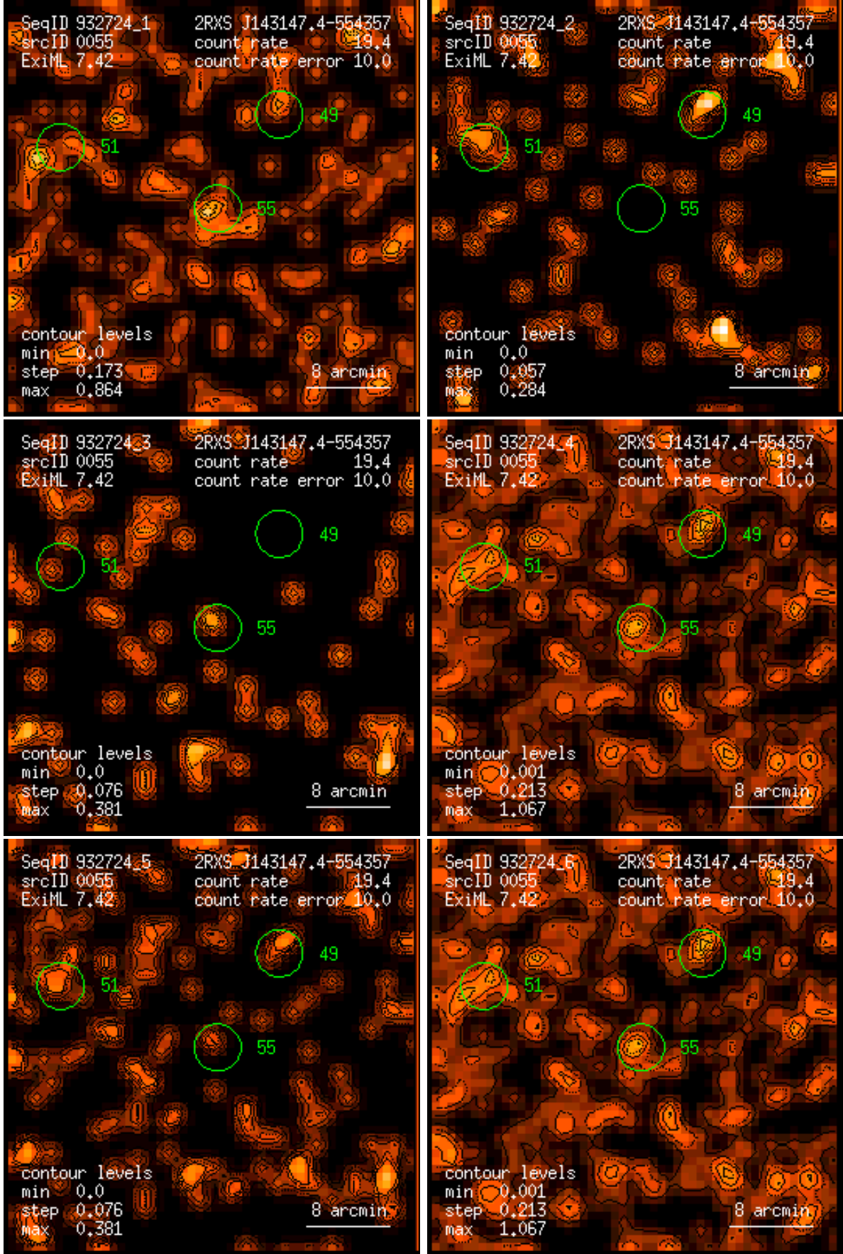
Figure 55: RASS 932724: detection 0055: band rate images, Gaussian filter: (1) PSPC channels 11 – 41, (2) 52 – 90, (3) 91 – 201, (4) 11 – 235, (5) 52 – 201, (6) 11 – 201. Broad band rates in counts/ks. Band rate contour levels in counts/ks/arcmin 2 .
