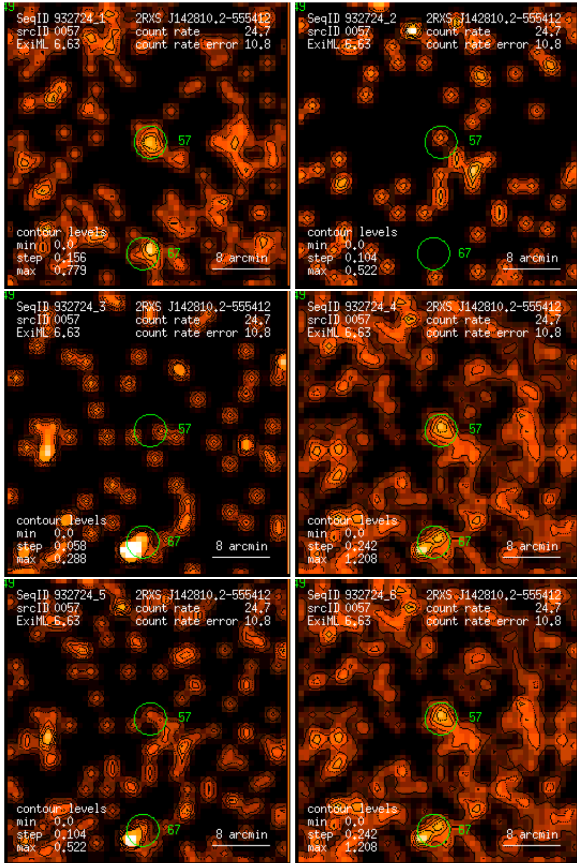
Figure 57: RASS 932724: detection 0057: band rate images, Gaussian filter: (1) PSPC channels 11 – 41, (2) 52 – 90, (3) 91 – 201, (4) 11 – 235, (5) 52 – 201, (6) 11 – 201. Broad band rates in counts/ks. Band rate contour levels in counts/ks/arcmin 2 .
