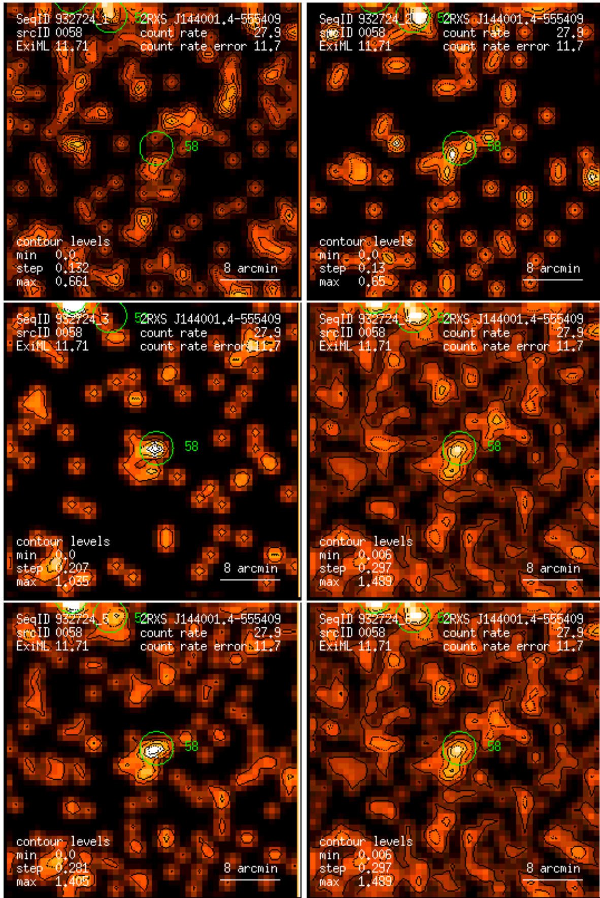
Figure 58: RASS 932724: detection 0058: band rate images, Gaussian filter: (1) PSPC channels 11 – 41, (2) 52 – 90, (3) 91 – 201, (4) 11 – 235, (5) 52 – 201, (6) 11 – 201. Broad band rates in counts/ks. Band rate contour levels in counts/ks/arcmin 2 .
