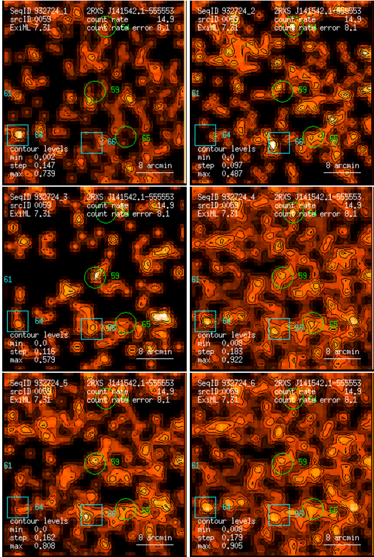
Figure 59: RASS 932724: detection 0059: band rate images, Gaussian filter: (1) PSPC channels 11 – 41, (2) 52 – 90, (3) 91 – 201, (4) 11 – 235, (5) 52 – 201, (6) 11 – 201. Broad band rates in counts/ks. Band rate contour levels in counts/ks/arcmin 2 .
