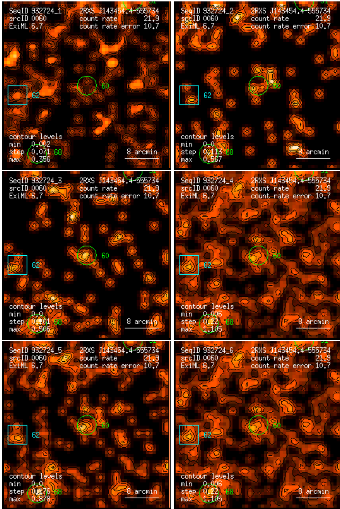
Figure 60: RASS 932724: detection 0060: band rate images, Gaussian filter: (1) PSPC channels 11 – 41, (2) 52 – 90, (3) 91 – 201, (4) 11 – 235, (5) 52 – 201, (6) 11 – 201. Broad band rates in counts/ks. Band rate contour levels in counts/ks/arcmin 2 .
