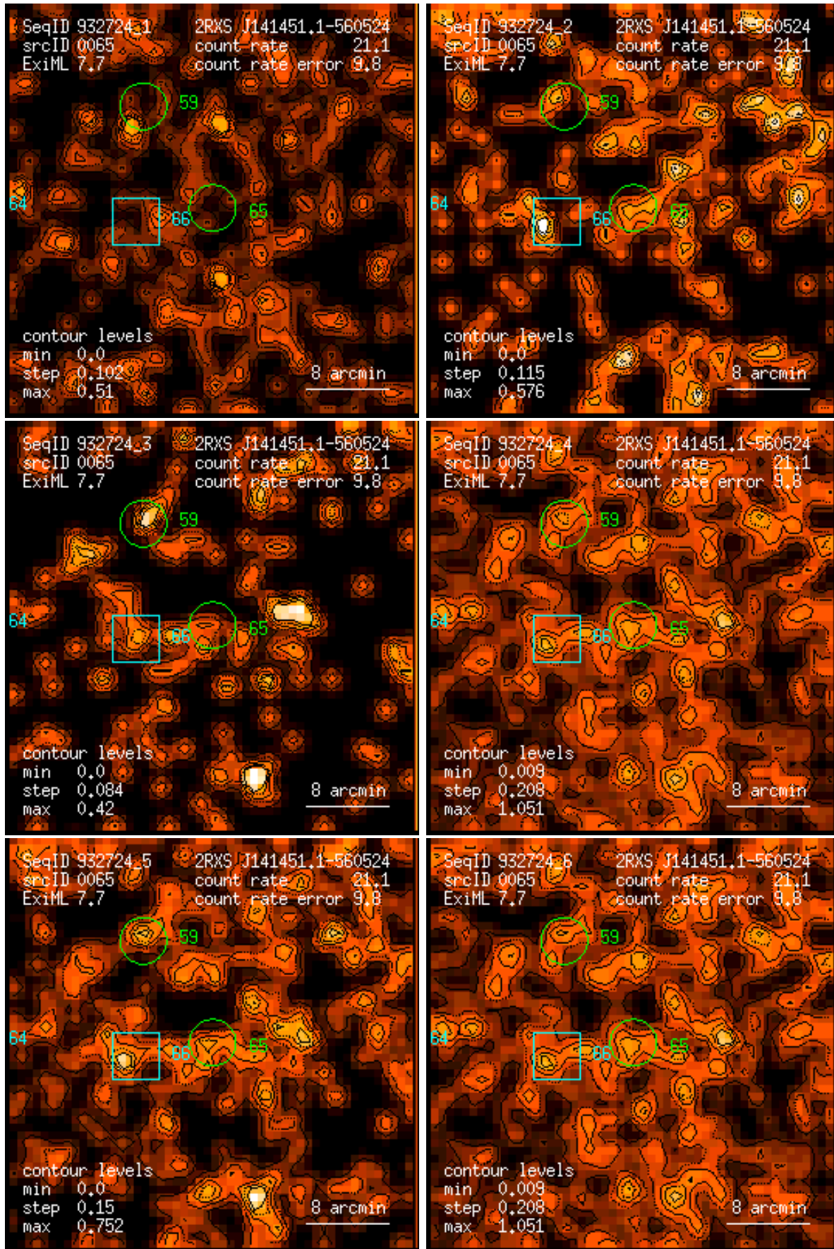
Figure 65: RASS 932724: detection 0065: band rate images, Gaussian filter: (1) PSPC channels 11 – 41, (2) 52 – 90, (3) 91 – 201, (4) 11 – 235, (5) 52 – 201, (6) 11 – 201. Broad band rates in counts/ks. Band rate contour levels in counts/ks/arcmin 2 .
