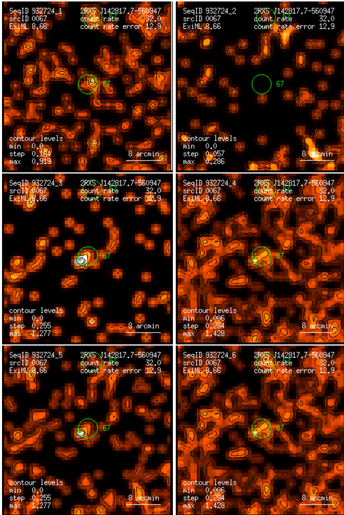
Figure 67: RASS 932724: detection 0067: band rate images, Gaussian filter: (1) PSPC channels 11 – 41, (2) 52 – 90, (3) 91 – 201, (4) 11 – 235, (5) 52 – 201, (6) 11 – 201. Broad band rates in counts/ks. Band rate contour levels in counts/ks/arcmin 2 .
