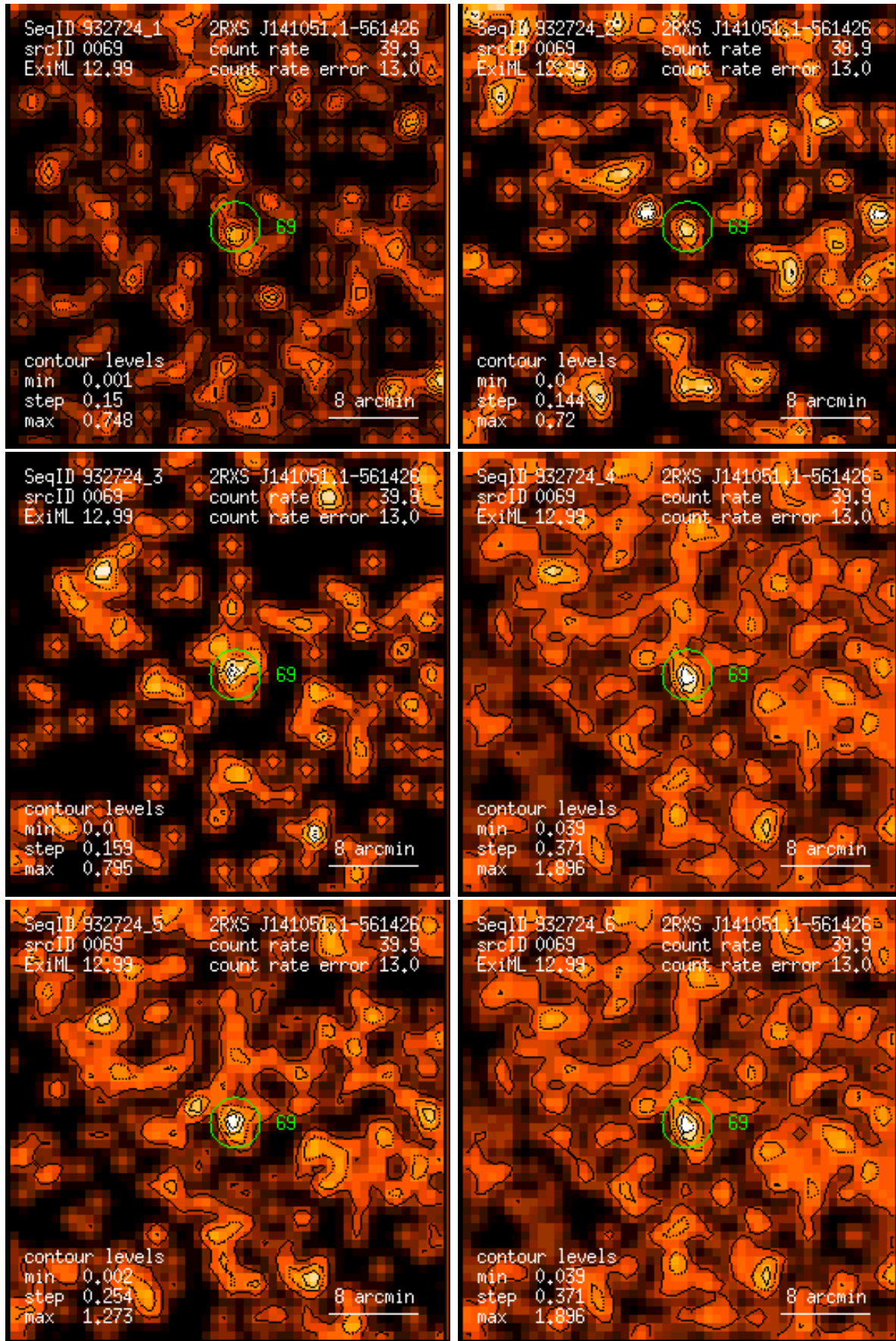
Figure 69: RASS 932724: detection 0069: band rate images, Gaussian filter: (1) PSPC channels 11 – 41, (2) 52 – 90, (3) 91 – 201, (4) 11 – 235, (5) 52 – 201, (6) 11 – 201. Broad band rates in counts/ks. Band rate contour levels in counts/ks/arcmin 2 .
