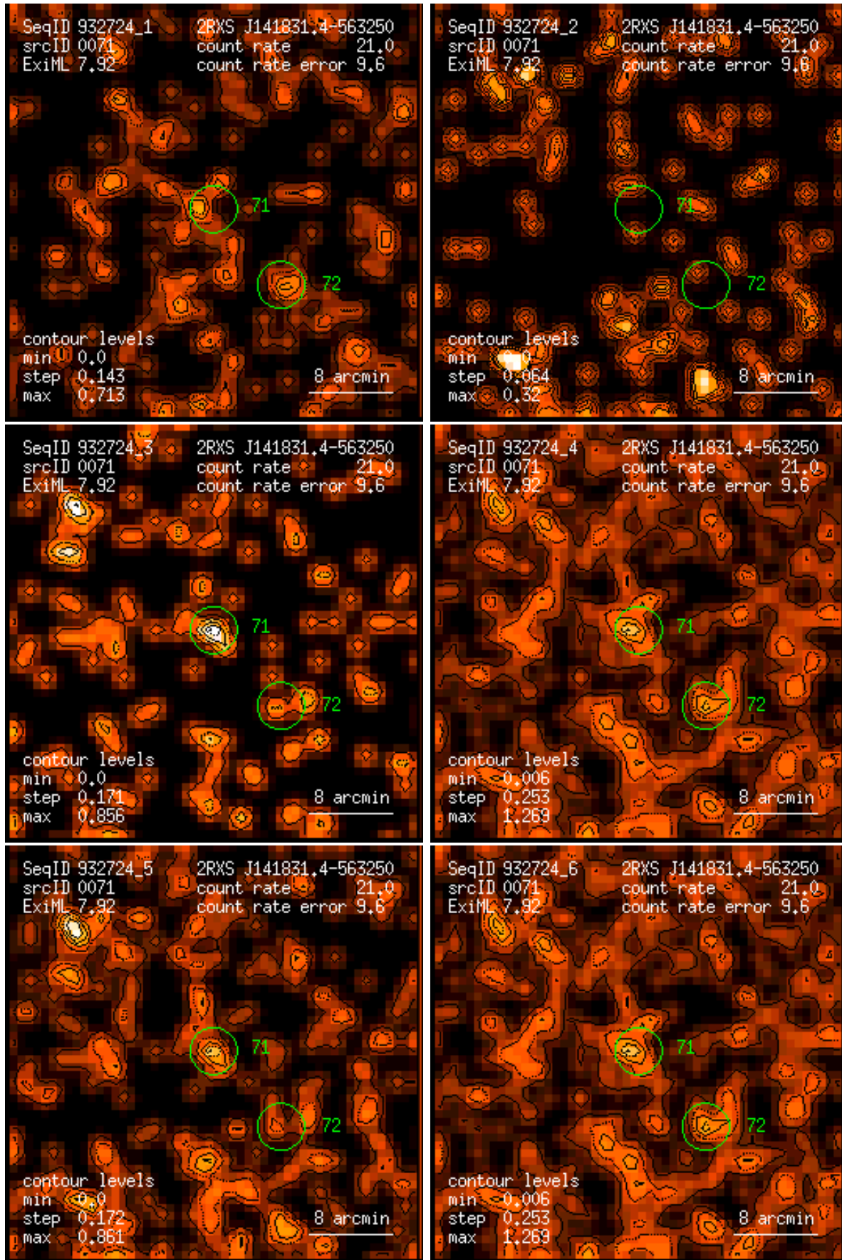
Figure 71: RASS 932724: detection 0071: band rate images, Gaussian filter: (1) PSPC channels 11 – 41, (2) 52 – 90, (3) 91 – 201, (4) 11 – 235, (5) 52 – 201, (6) 11 – 201. Broad band rates in counts/ks. Band rate contour levels in counts/ks/arcmin 2 .
