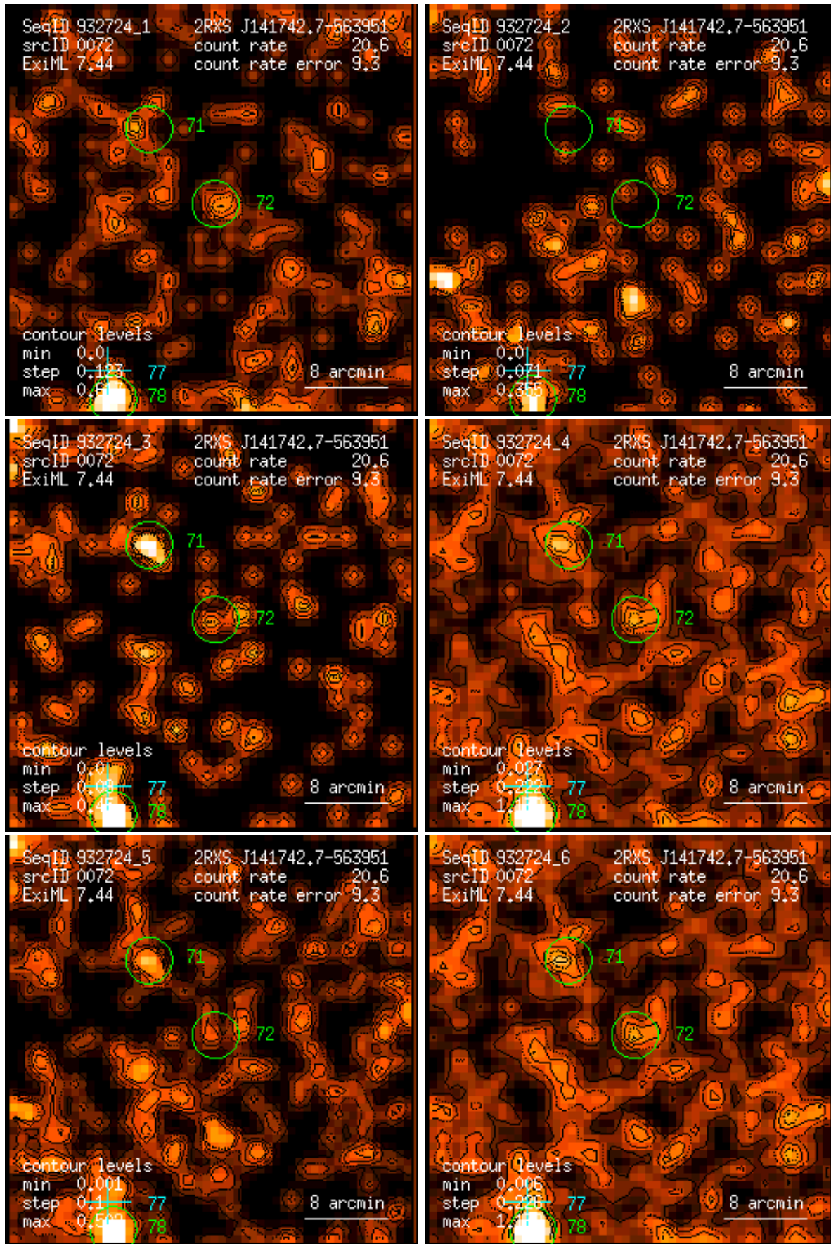
Figure 72: RASS 932724: detection 0072: band rate images, Gaussian filter: (1) PSPC channels 11 – 41, (2) 52 – 90, (3) 91 – 201, (4) 11 – 235, (5) 52 – 201, (6) 11 – 201. Broad band rates in counts/ks. Band rate contour levels in counts/ks/arcmin 2 .
