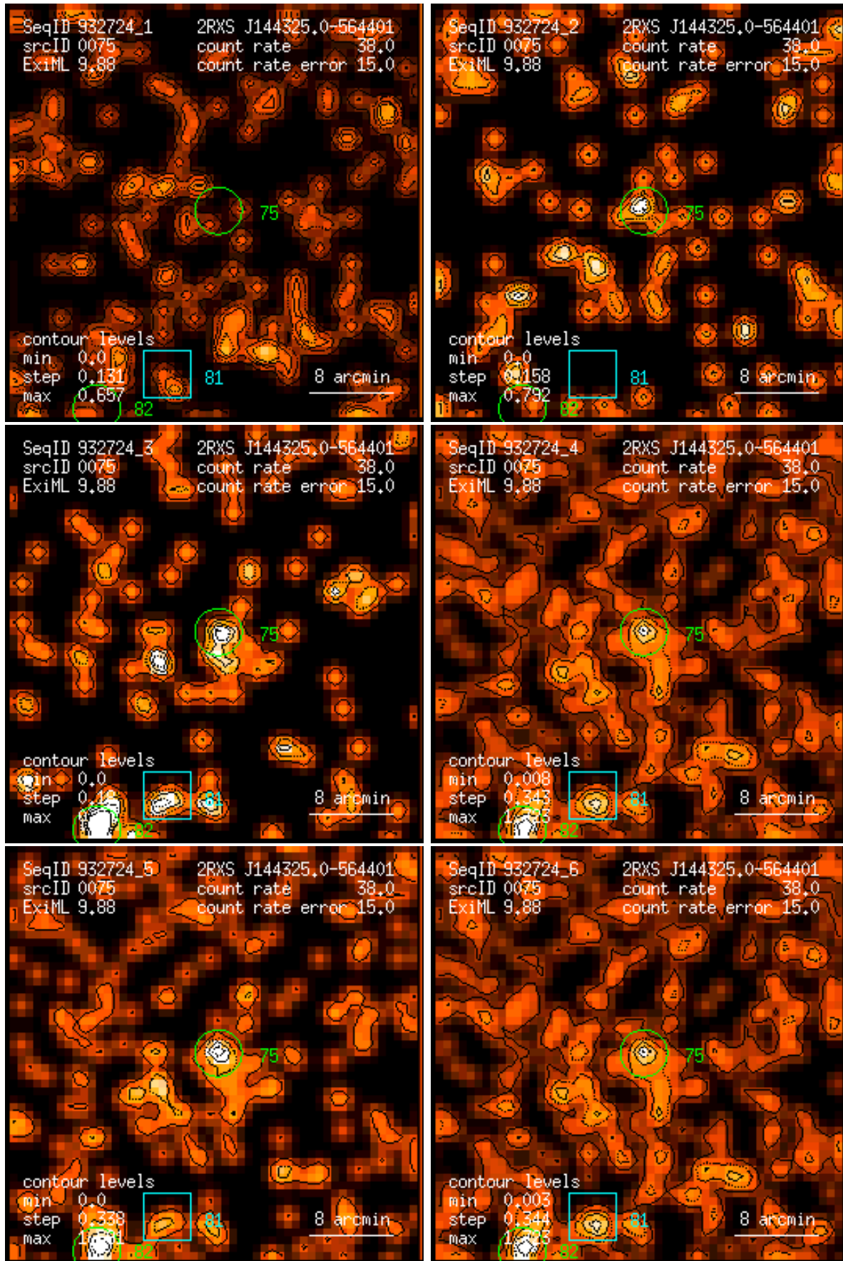
Figure 75: RASS 932724: detection 0075: band rate images, Gaussian filter: (1) PSPC channels 11 – 41, (2) 52 – 90, (3) 91 – 201, (4) 11 – 235, (5) 52 – 201, (6) 11 – 201. Broad band rates in counts/ks. Band rate contour levels in counts/ks/arcmin 2 .
