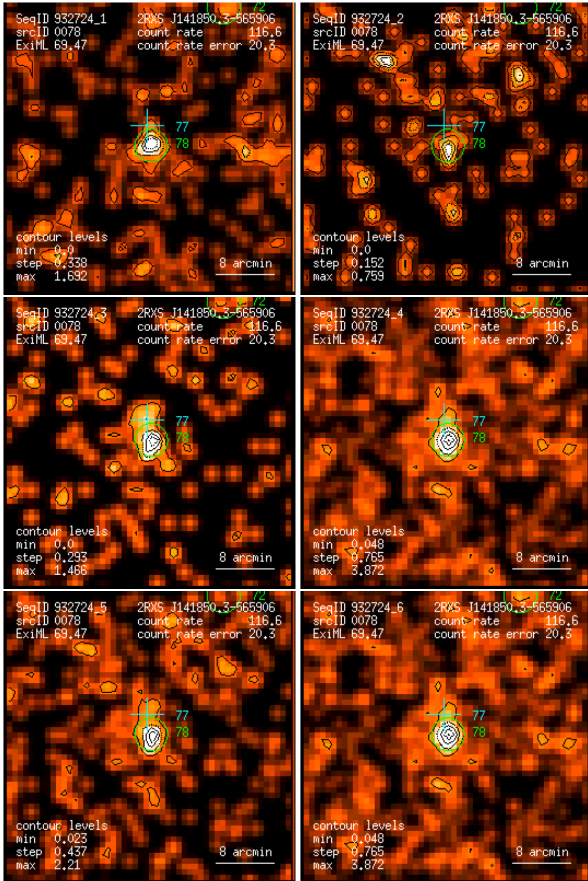
Figure 78: RASS 932724: detection 0078: band rate images, Gaussian filter: (1) PSPC channels 11 – 41, (2) 52 – 90, (3) 91 – 201, (4) 11 – 235, (5) 52 – 201, (6) 11 – 201. Broad band rates in counts/ks. Band rate contour levels in counts/ks/arcmin 2 .
