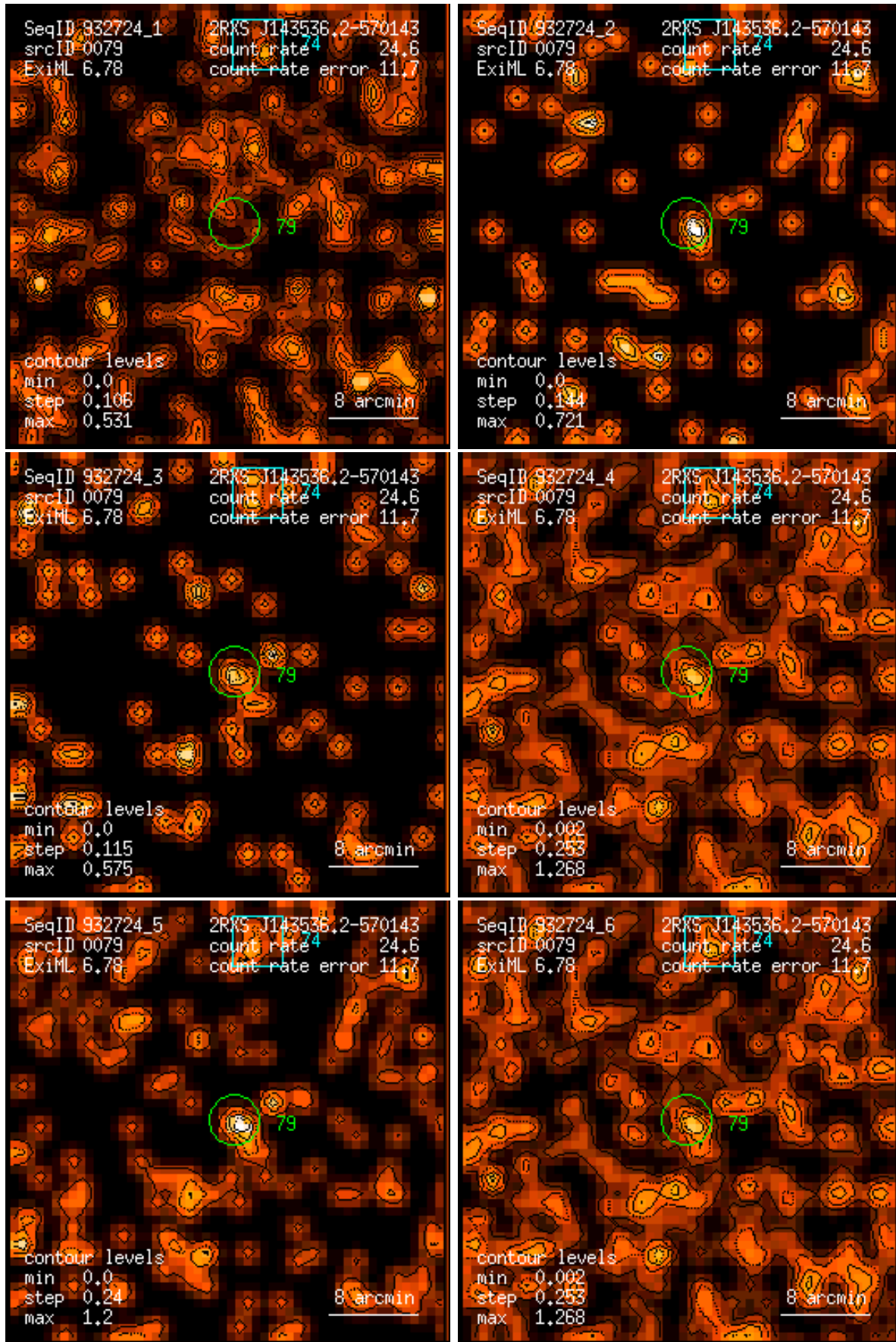
Figure 79: RASS 932724: detection 0079: band rate images, Gaussian filter: (1) PSPC channels 11 – 41, (2) 52 – 90, (3) 91 – 201, (4) 11 – 235, (5) 52 – 201, (6) 11 – 201. Broad band rates in counts/ks. Band rate contour levels in counts/ks/arcmin 2 .
