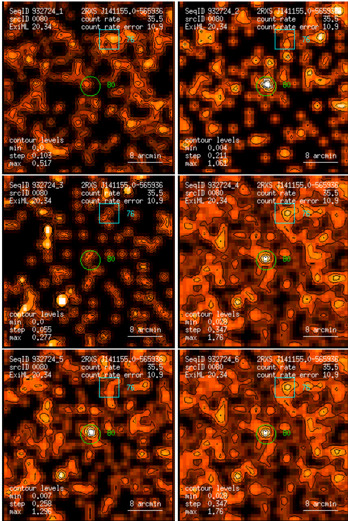
Figure 80: RASS 932724: detection 0080: band rate images, Gaussian filter: (1) PSPC channels 11 – 41, (2) 52 – 90, (3) 91 – 201, (4) 11 – 235, (5) 52 – 201, (6) 11 – 201. Broad band rates in counts/ks. Band rate contour levels in counts/ks/arcmin 2 .
