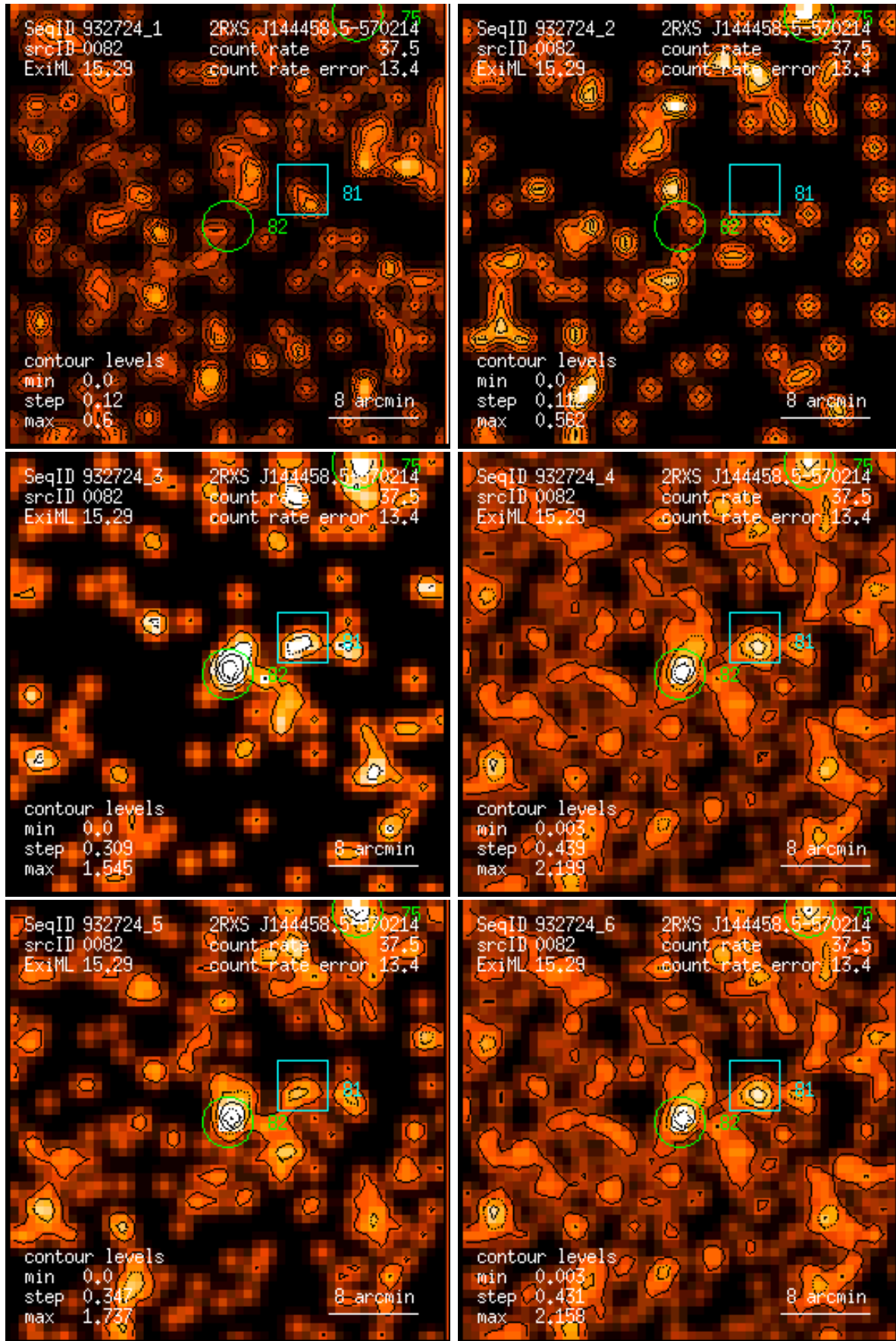
Figure 82: RASS 932724: detection 0082: band rate images, Gaussian filter: (1) PSPC channels 11 – 41, (2) 52 – 90, (3) 91 – 201, (4) 11 – 235, (5) 52 – 201, (6) 11 – 201. Broad band rates in counts/ks. Band rate contour levels in counts/ks/arcmin 2 .
