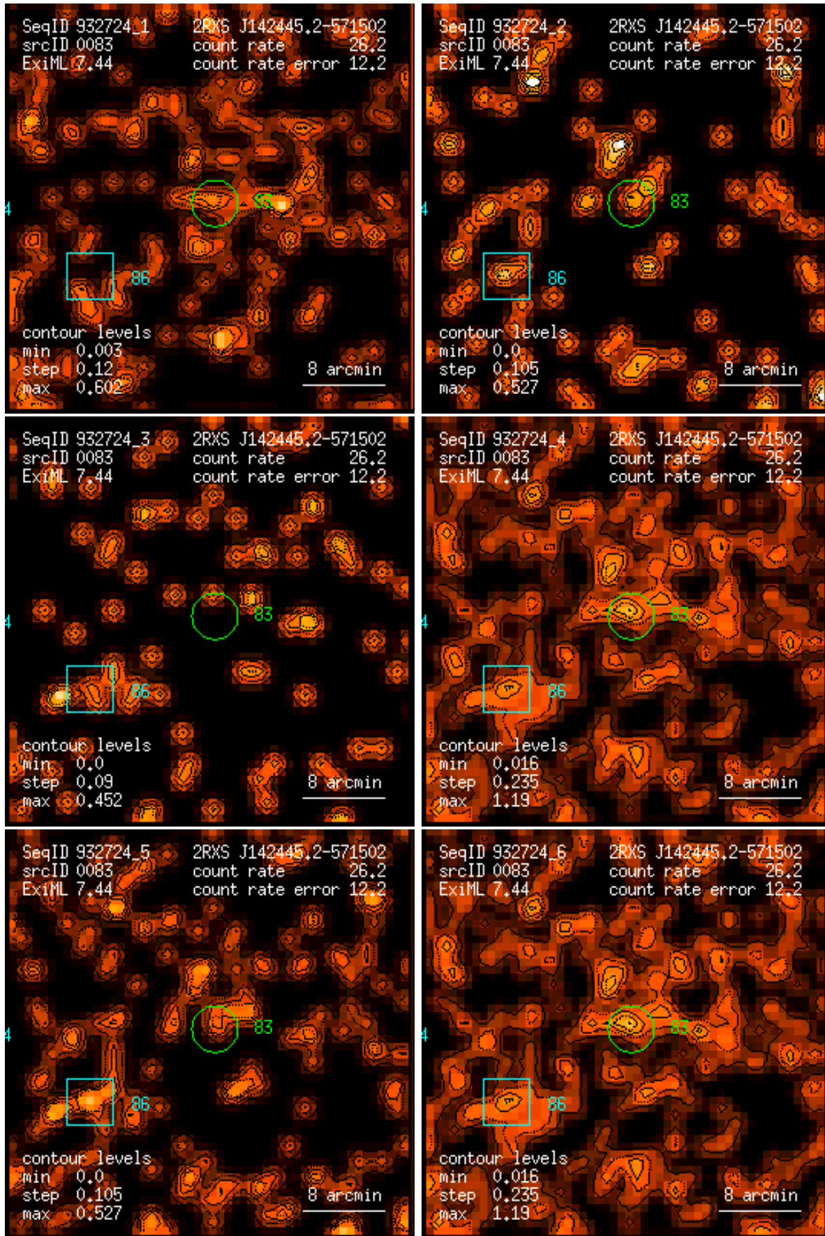
Figure 83: RASS 932724: detection 0083: band rate images, Gaussian filter: (1) PSPC channels 11 – 41, (2) 52 – 90, (3) 91 – 201, (4) 11 – 235, (5) 52 – 201, (6) 11 – 201. Broad band rates in counts/ks. Band rate contour levels in counts/ks/arcmin 2 .
