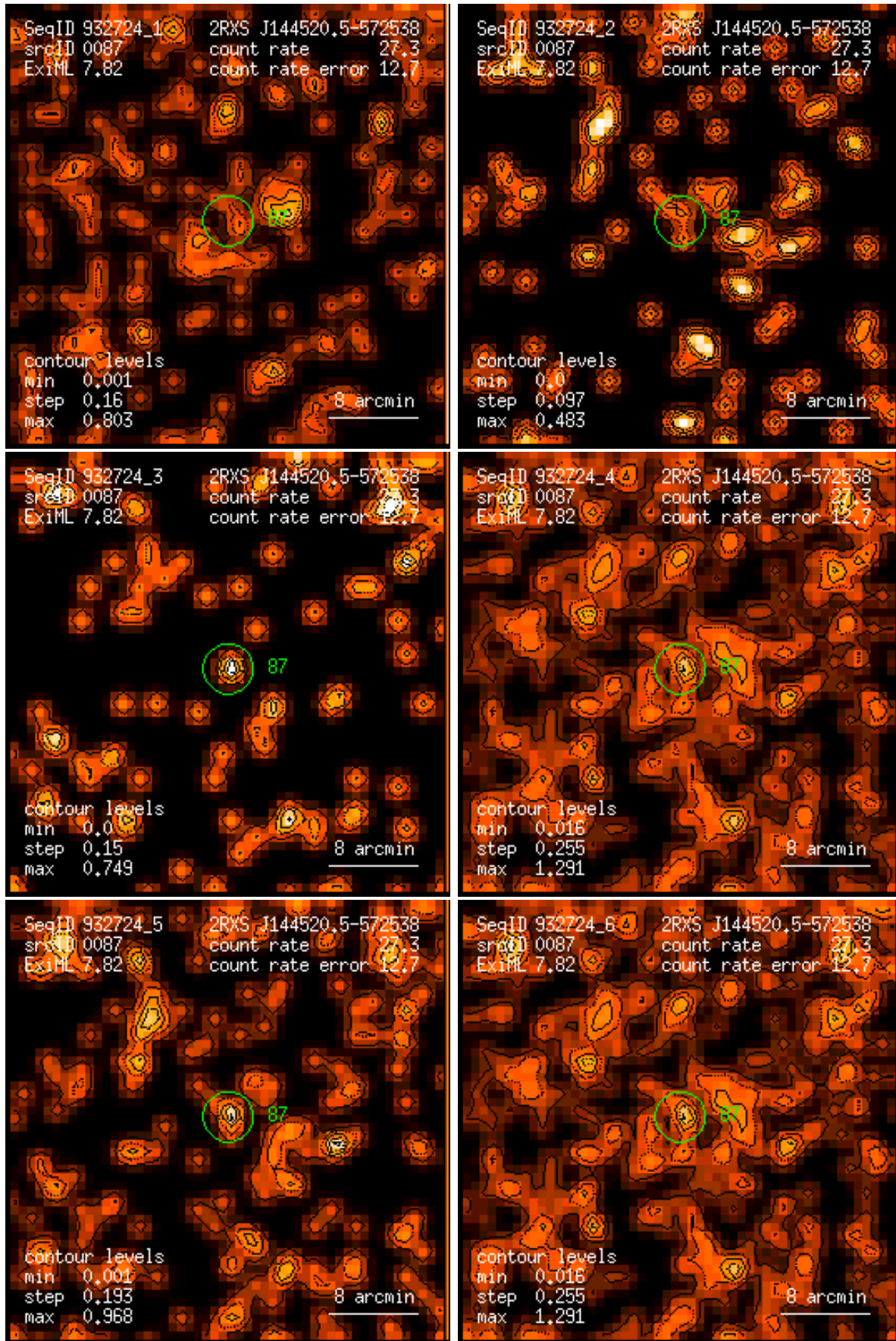
Figure 87: RASS 932724: detection 0087: band rate images, Gaussian filter: (1) PSPC channels 11 – 41, (2) 52 – 90, (3) 91 – 201, (4) 11 – 235, (5) 52 – 201, (6) 11 – 201. Broad band rates in counts/ks. Band rate contour levels in counts/ks/arcmin 2 .
