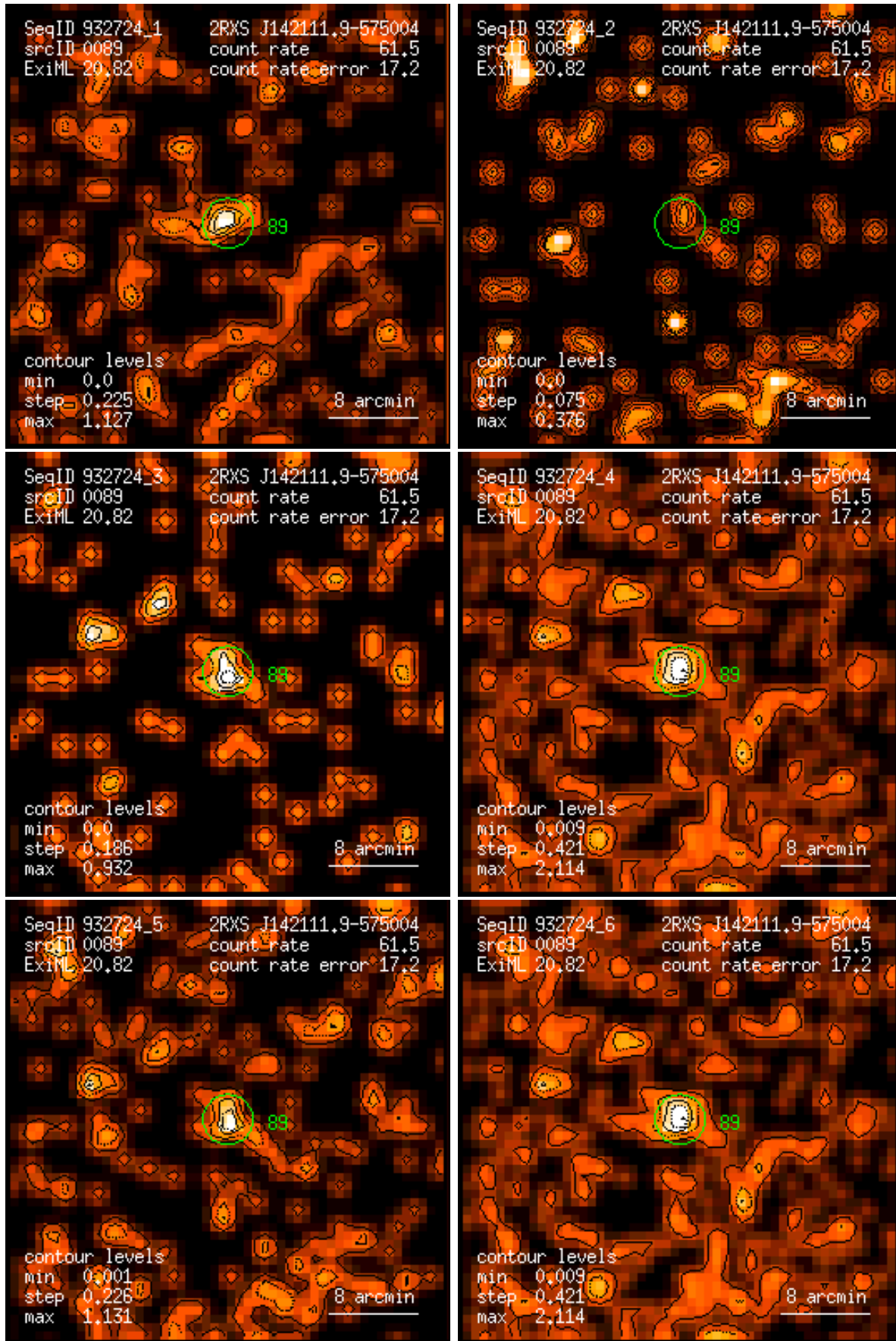
Figure 89: RASS 932724: detection 0089: band rate images, Gaussian filter: (1) PSPC channels 11 – 41, (2) 52 – 90, (3) 91 – 201, (4) 11 – 235, (5) 52 – 201, (6) 11 – 201. Broad band rates in counts/ks. Band rate contour levels in counts/ks/arcmin 2 .
