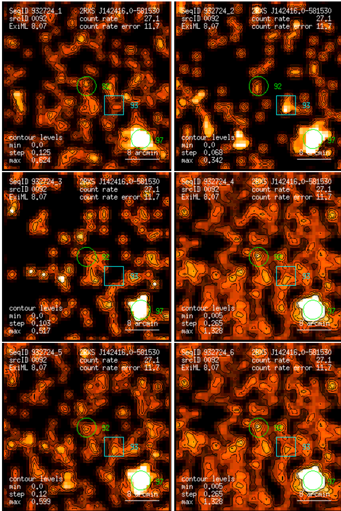
Figure 92: RASS 932724: detection 0092: band rate images, Gaussian filter: (1) PSPC channels 11 – 41, (2) 52 – 90, (3) 91 – 201, (4) 11 – 235, (5) 52 – 201, (6) 11 – 201. Broad band rates in counts/ks. Band rate contour levels in counts/ks/arcmin 2 .
