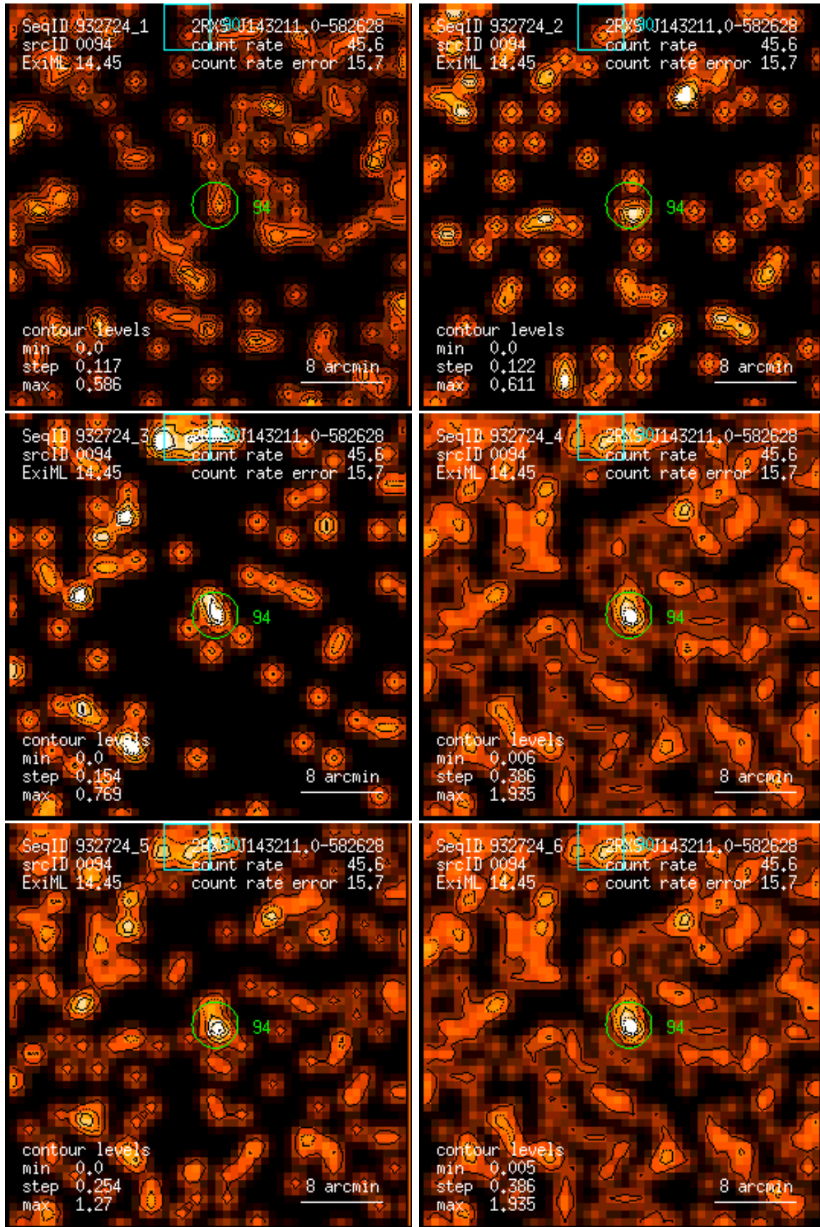
Figure 94: RASS 932724: detection 0094: band rate images, Gaussian filter: (1) PSPC channels 11 – 41, (2) 52 – 90, (3) 91 – 201, (4) 11 – 235, (5) 52 – 201, (6) 11 – 201. Broad band rates in counts/ks. Band rate contour levels in counts/ks/arcmin 2 .
