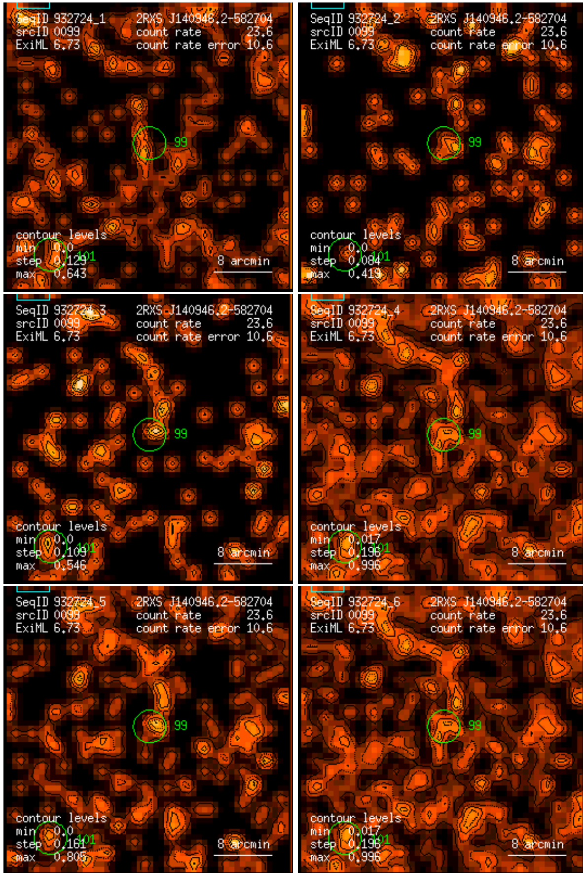
Figure 99: RASS 932724: detection 0099: band rate images, Gaussian filter: (1) PSPC channels 11 – 41, (2) 52 – 90, (3) 91 – 201, (4) 11 – 235, (5) 52 – 201, (6) 11 – 201. Broad band rates in counts/ks. Band rate contour levels in counts/ks/arcmin 2 .
