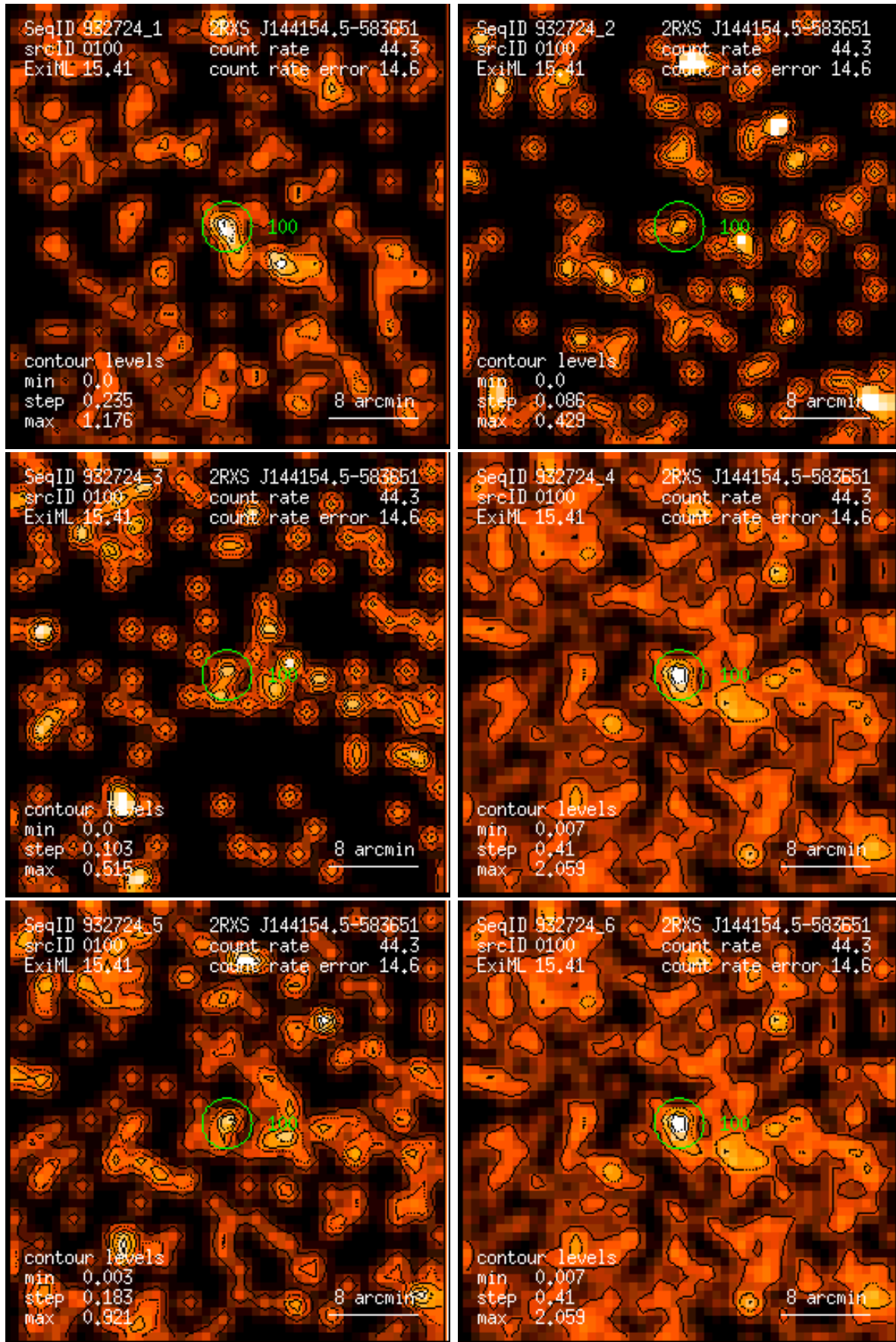
Figure 100: RASS 932724: detection 0100: band rate images, Gaussian filter: (1) PSPC channels 11 – 41, (2) 52 – 90, (3) 91 – 201, (4) 11 – 235, (5) 52 – 201, (6) 11 – 201. Broad band rates in counts/ks. Band rate contour levels in counts/ks/arcmin 2 .
