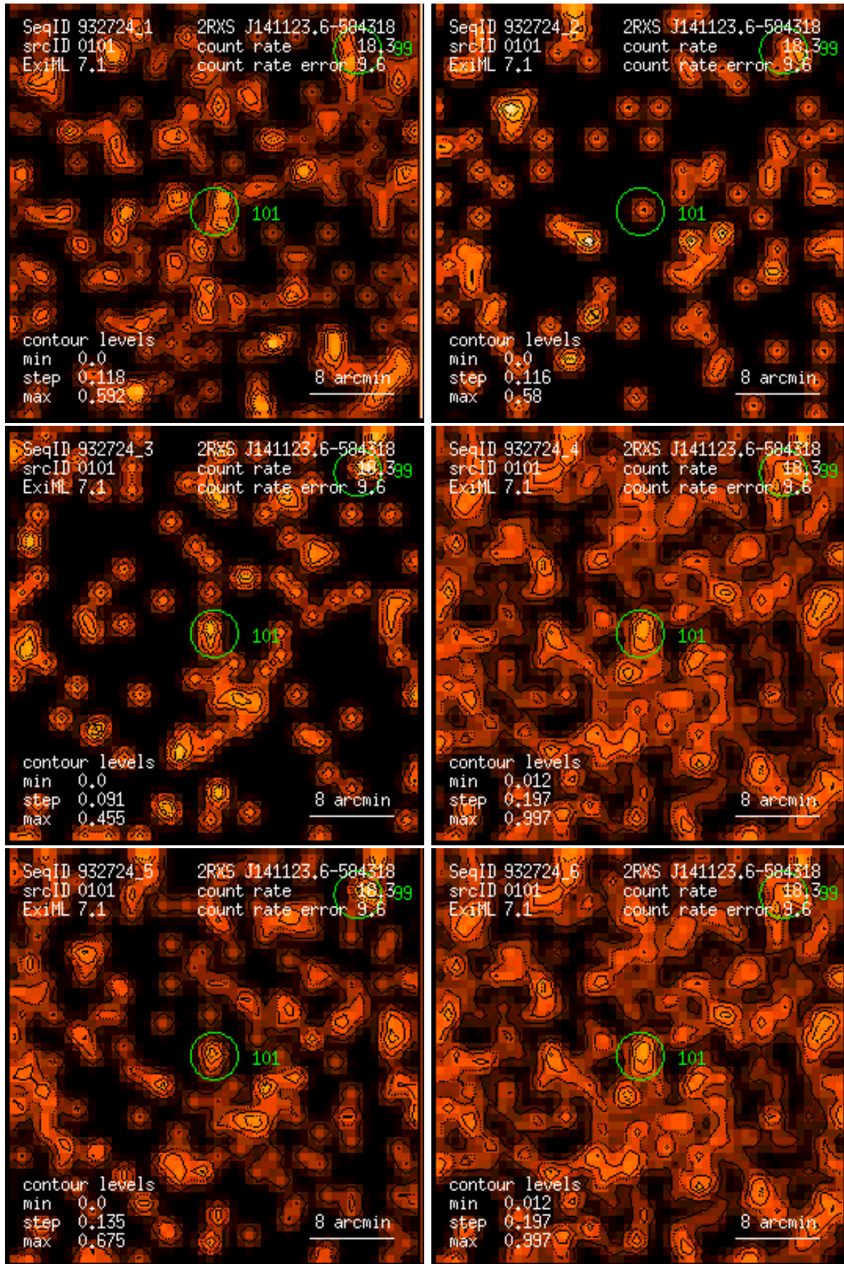
Figure 101: RASS 932724: detection 0101: band rate images, Gaussian filter: (1) PSPC channels 11 – 41, (2) 52 – 90, (3) 91 – 201, (4) 11 – 235, (5) 52 – 201, (6) 11 – 201. Broad band rates in counts/ks. Band rate contour levels in counts/ks/arcmin 2 .
