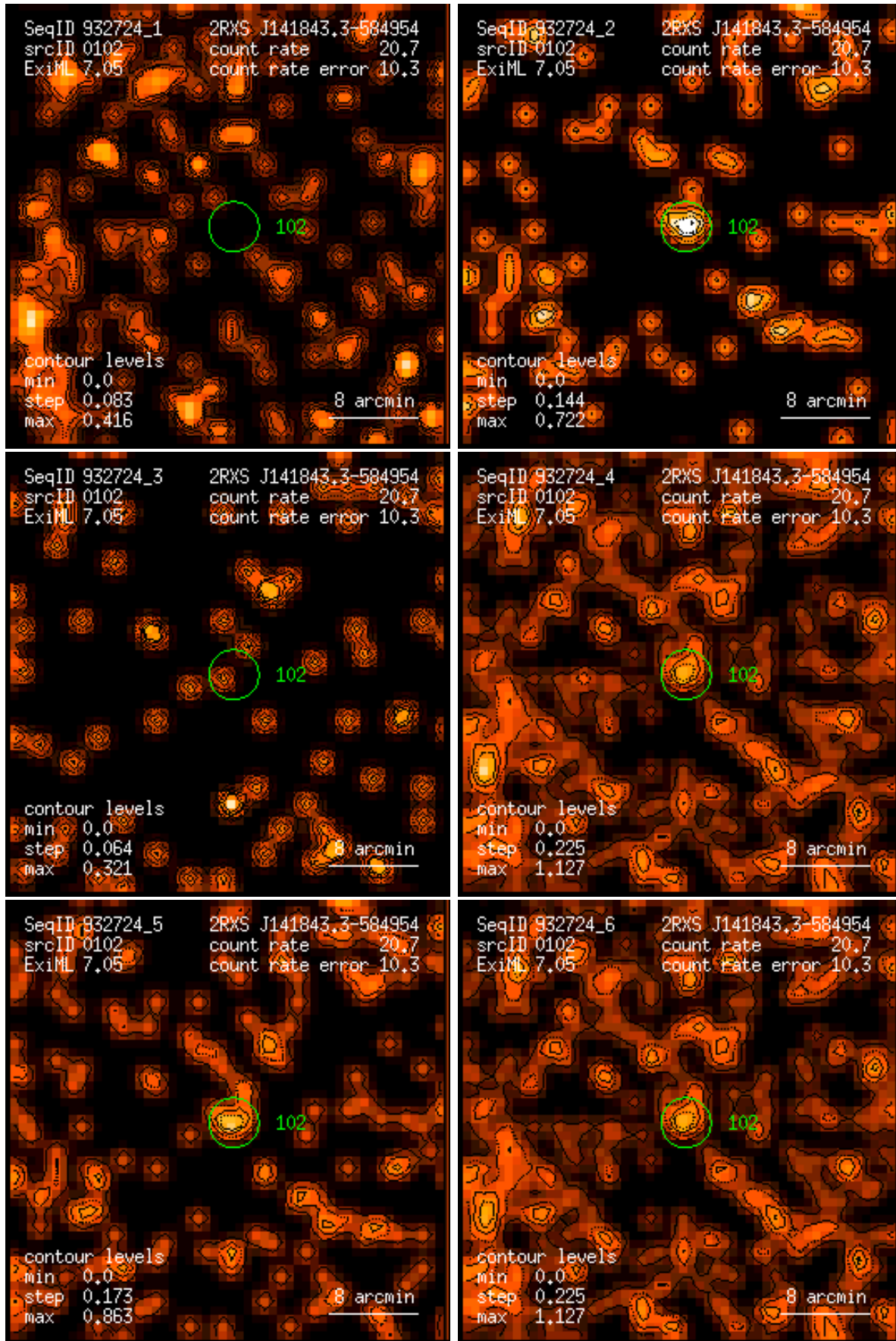
Figure 102: RASS 932724: detection 0102: band rate images, Gaussian filter: (1) PSPC channels 11 – 41, (2) 52 – 90, (3) 91 – 201, (4) 11 – 235, (5) 52 – 201, (6) 11 – 201. Broad band rates in counts/ks. Band rate contour levels in counts/ks/arcmin 2 .
