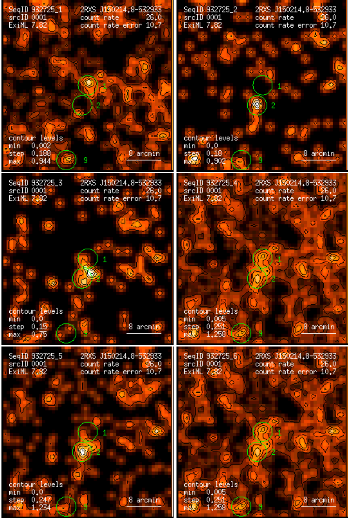
Figure 1: RASS 932725: detection 0001: band rate images, Gaussian filter: (1) PSPC channels 11 – 41, (2) 52 – 90, (3) 91 – 201, (4) 11 – 235, (5) 52 – 201, (6) 11 – 201. Broad band rates in counts/ks. Band rate contour levels in counts/ks/arcmin 2 .
