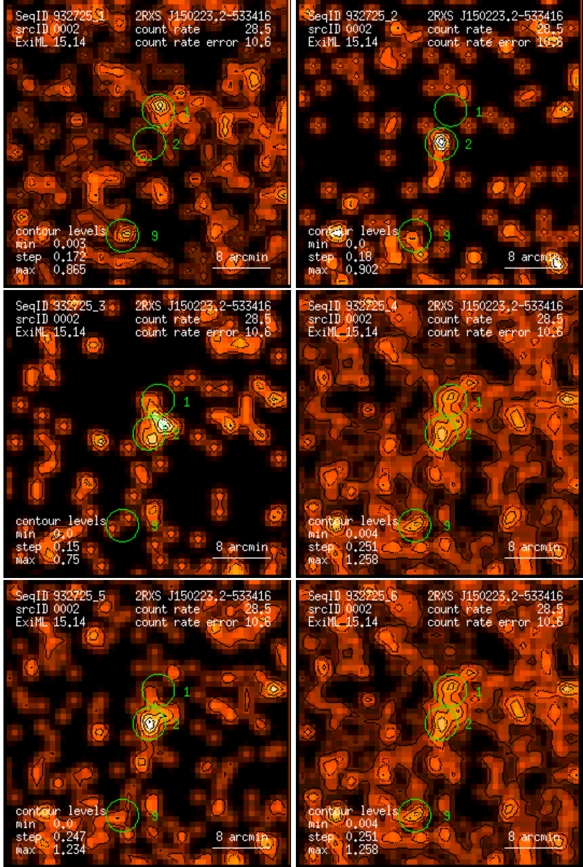
Figure 2: RASS 932725: detection 0002: band rate images, Gaussian filter: (1) PSPC channels 11 – 41, (2) 52 – 90, (3) 91 – 201, (4) 11 – 235, (5) 52 – 201, (6) 11 – 201. Broad band rates in counts/ks. Band rate contour levels in counts/ks/arcmin 2 .
