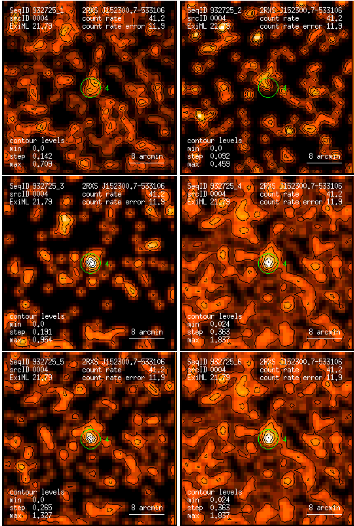
Figure 4: RASS 932725: detection 0004: band rate images, Gaussian filter: (1) PSPC channels 11 – 41, (2) 52 – 90, (3) 91 – 201, (4) 11 – 235, (5) 52 – 201, (6) 11 – 201. Broad band rates in counts/ks. Band rate contour levels in counts/ks/arcmin 2 .
