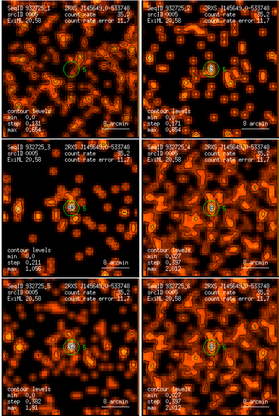
Figure 5: RASS 932725: detection 0005: band rate images, Gaussian filter: (1) PSPC channels 11 – 41, (2) 52 – 90, (3) 91 – 201, (4) 11 – 235, (5) 52 – 201, (6) 11 – 201. Broad band rates in counts/ks. Band rate contour levels in counts/ks/arcmin 2 .
