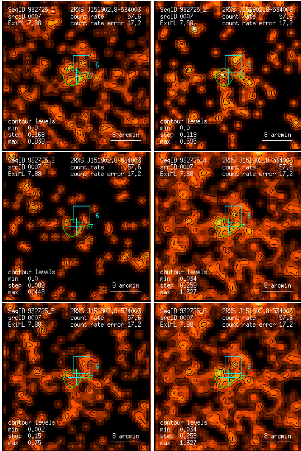
Figure 7: RASS 932725: detection 0007: band rate images, Gaussian filter: (1) PSPC channels 11 – 41, (2) 52 – 90, (3) 91 – 201, (4) 11 – 235, (5) 52 – 201, (6) 11 – 201. Broad band rates in counts/ks. Band rate contour levels in counts/ks/arcmin 2 .
