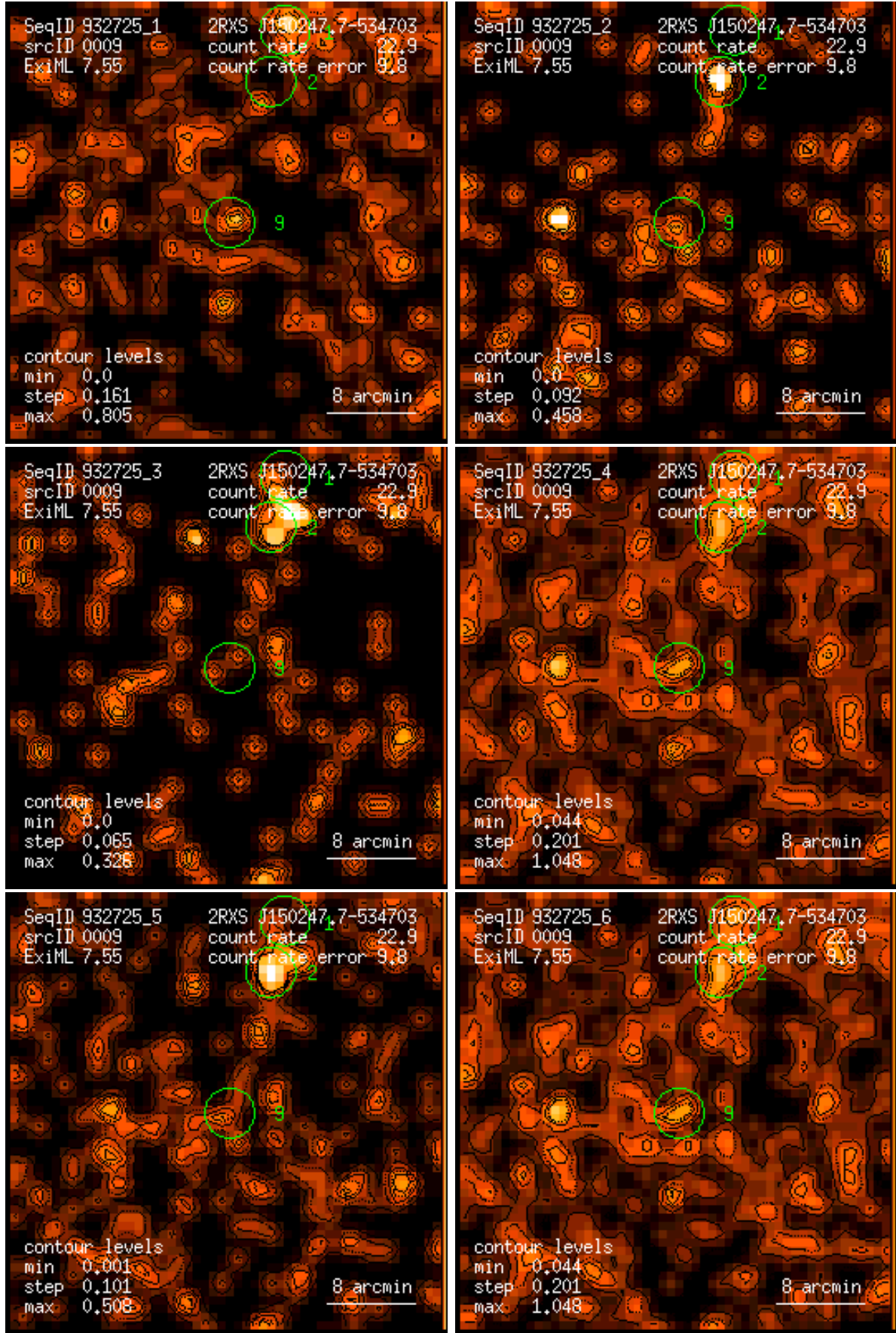
Figure 9: RASS 932725: detection 0009: band rate images, Gaussian filter: (1) PSPC channels 11 – 41, (2) 52 – 90, (3) 91 – 201, (4) 11 – 235, (5) 52 – 201, (6) 11 – 201. Broad band rates in counts/ks. Band rate contour levels in counts/ks/arcmin 2 .
