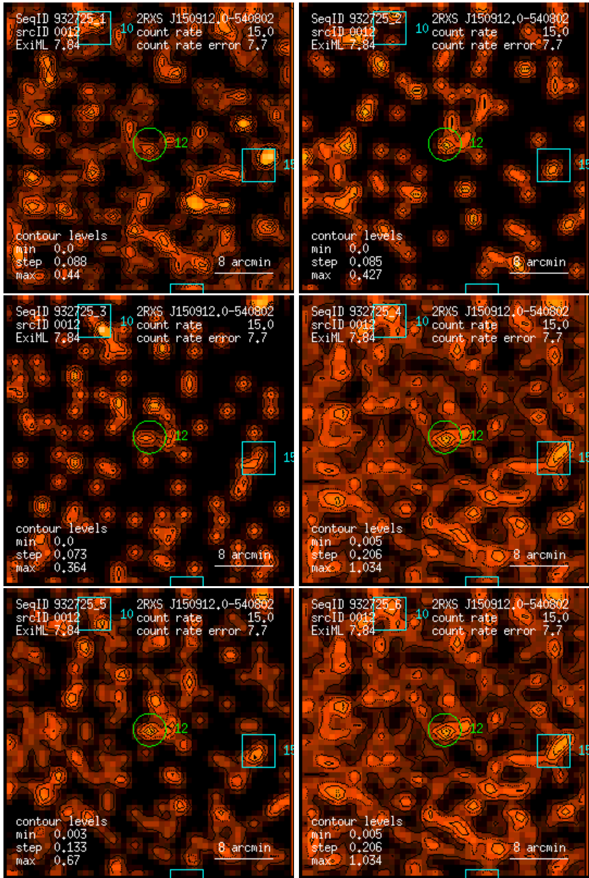
Figure 12: RASS 932725: detection 0012: band rate images, Gaussian filter: (1) PSPC channels 11 – 41, (2) 52 – 90, (3) 91 – 201, (4) 11 – 235, (5) 52 – 201, (6) 11 – 201. Broad band rates in counts/ks. Band rate contour levels in counts/ks/arcmin 2 .
