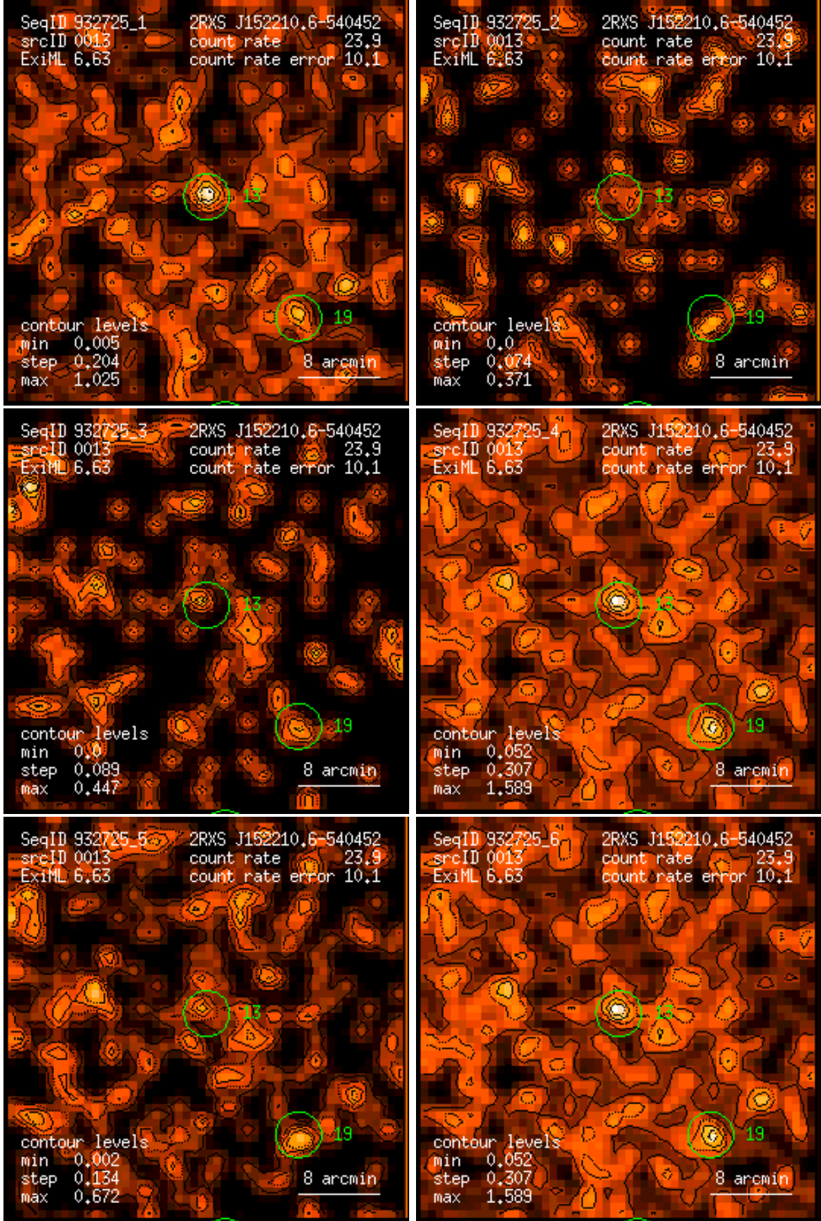
Figure 13: RASS 932725: detection 0013: band rate images, Gaussian filter: (1) PSPC channels 11 – 41, (2) 52 – 90, (3) 91 – 201, (4) 11 – 235, (5) 52 – 201, (6) 11 – 201. Broad band rates in counts/ks. Band rate contour levels in counts/ks/arcmin 2 .
