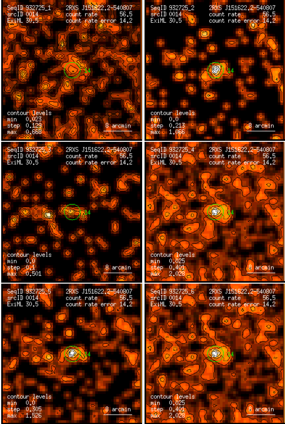
Figure 14: RASS 932725: detection 0014: band rate images, Gaussian filter: (1) PSPC channels 11 – 41, (2) 52 – 90, (3) 91 – 201, (4) 11 – 235, (5) 52 – 201, (6) 11 – 201. Broad band rates in counts/ks. Band rate contour levels in counts/ks/arcmin 2 .
