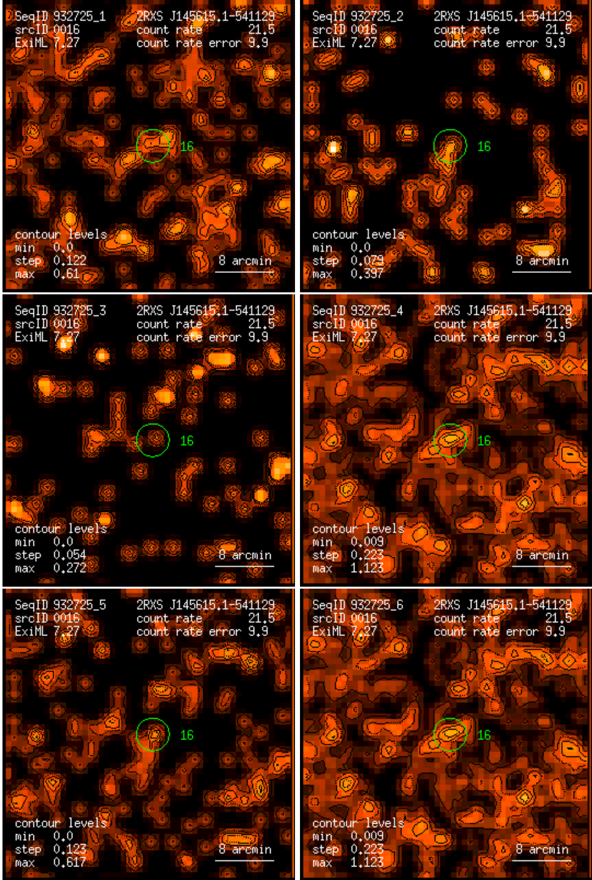
Figure 16: RASS 932725: detection 0016: band rate images, Gaussian filter: (1) PSPC channels 11 – 41, (2) 52 – 90, (3) 91 – 201, (4) 11 – 235, (5) 52 – 201, (6) 11 – 201. Broad band rates in counts/ks. Band rate contour levels in counts/ks/arcmin 2 .
