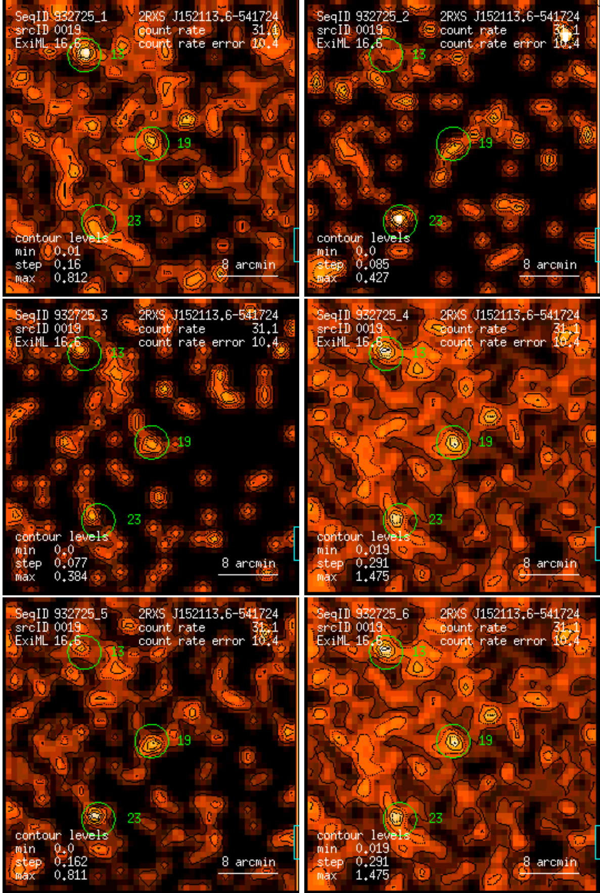
Figure 19: RASS 932725: detection 0019: band rate images, Gaussian filter: (1) PSPC channels 11 – 41, (2) 52 – 90, (3) 91 – 201, (4) 11 – 235, (5) 52 – 201, (6) 11 – 201. Broad band rates in counts/ks. Band rate contour levels in counts/ks/arcmin 2 .
