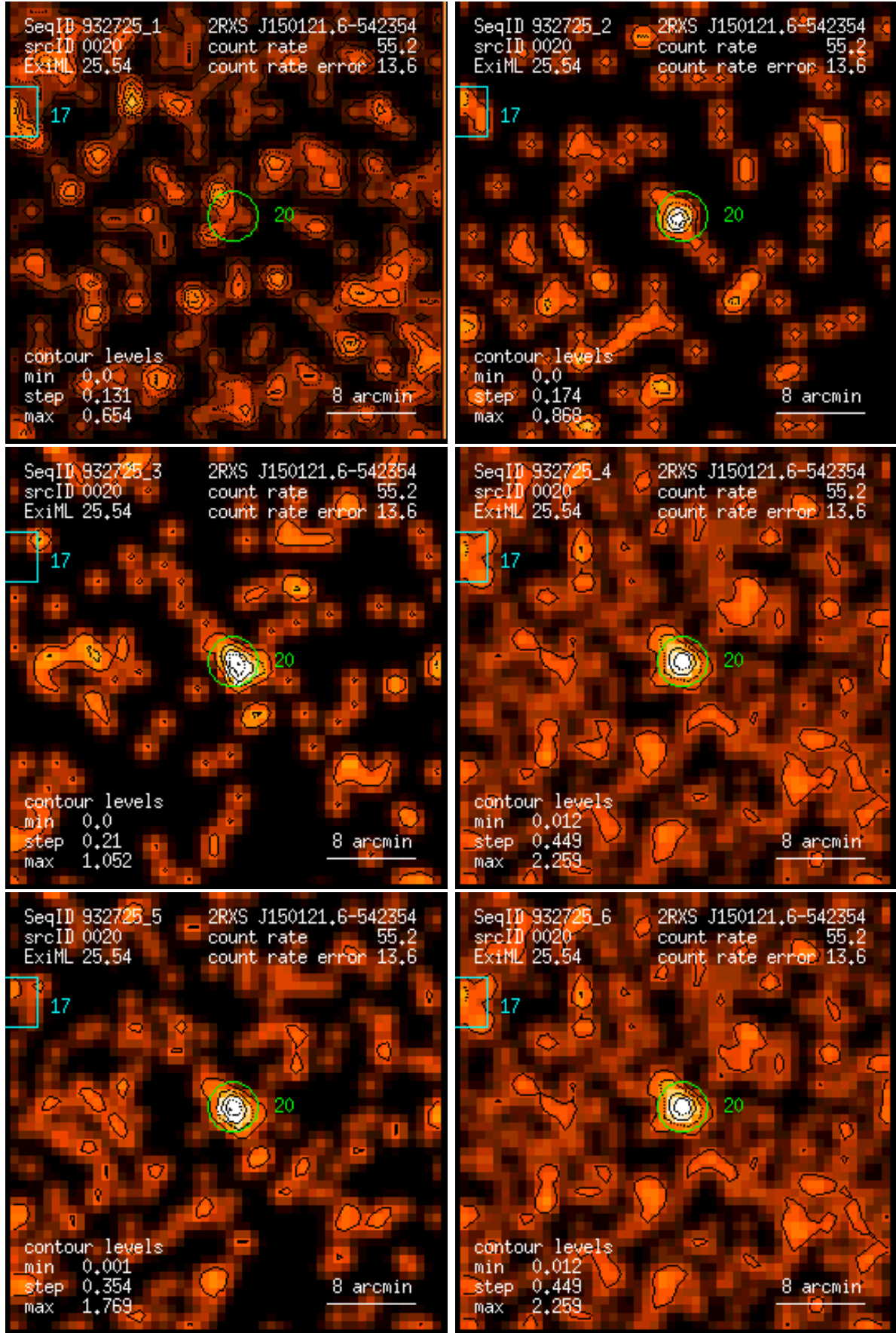
Figure 20: RASS 932725: detection 0020: band rate images, Gaussian filter: (1) PSPC channels 11 – 41, (2) 52 – 90, (3) 91 – 201, (4) 11 – 235, (5) 52 – 201, (6) 11 – 201. Broad band rates in counts/ks. Band rate contour levels in counts/ks/arcmin 2 .
