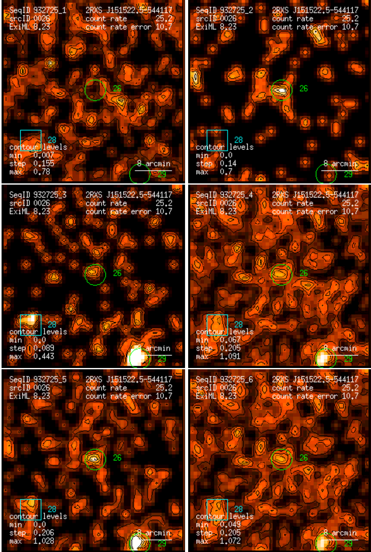
Figure 26: RASS 932725: detection 0026: band rate images, Gaussian filter: (1) PSPC channels 11 – 41, (2) 52 – 90, (3) 91 – 201, (4) 11 – 235, (5) 52 – 201, (6) 11 – 201. Broad band rates in counts/ks. Band rate contour levels in counts/ks/arcmin 2 .
