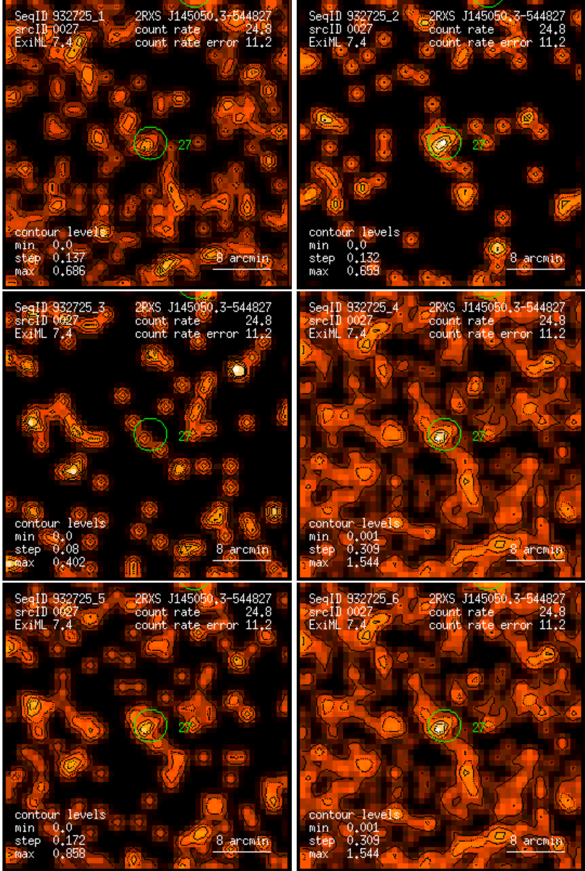
Figure 27: RASS 932725: detection 0027: band rate images, Gaussian filter: (1) PSPC channels 11 – 41, (2) 52 – 90, (3) 91 – 201, (4) 11 – 235, (5) 52 – 201, (6) 11 – 201. Broad band rates in counts/ks. Band rate contour levels in counts/ks/arcmin 2 .
