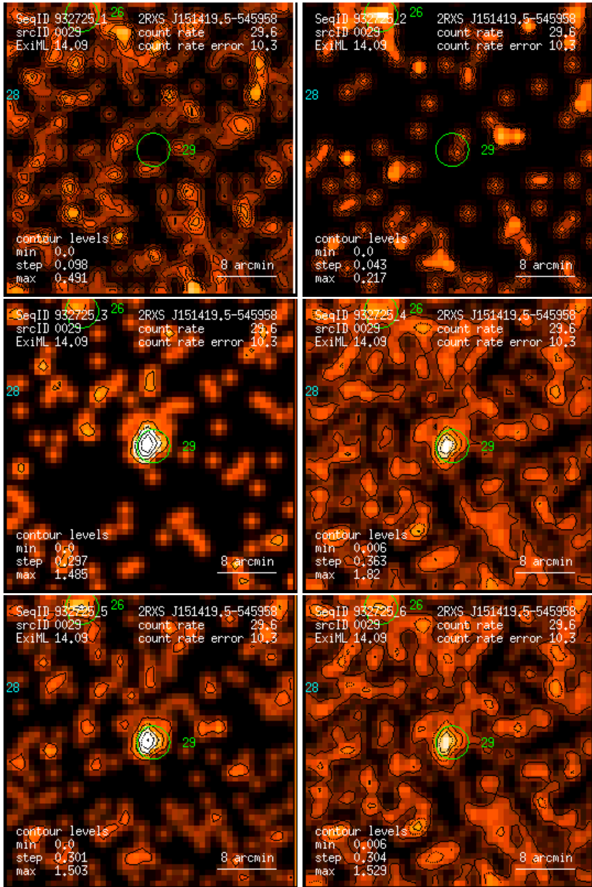
Figure 29: RASS 932725: detection 0029: band rate images, Gaussian filter: (1) PSPC channels 11 – 41, (2) 52 – 90, (3) 91 – 201, (4) 11 – 235, (5) 52 – 201, (6) 11 – 201. Broad band rates in counts/ks. Band rate contour levels in counts/ks/arcmin 2 .
