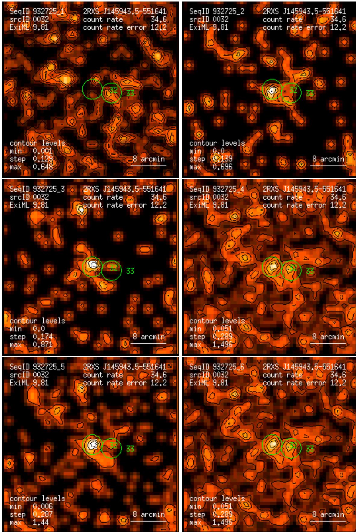
Figure 32: RASS 932725: detection 0032: band rate images, Gaussian filter: (1) PSPC channels 11 – 41, (2) 52 – 90, (3) 91 – 201, (4) 11 – 235, (5) 52 – 201, (6) 11 – 201. Broad band rates in counts/ks. Band rate contour levels in counts/ks/arcmin 2 .
