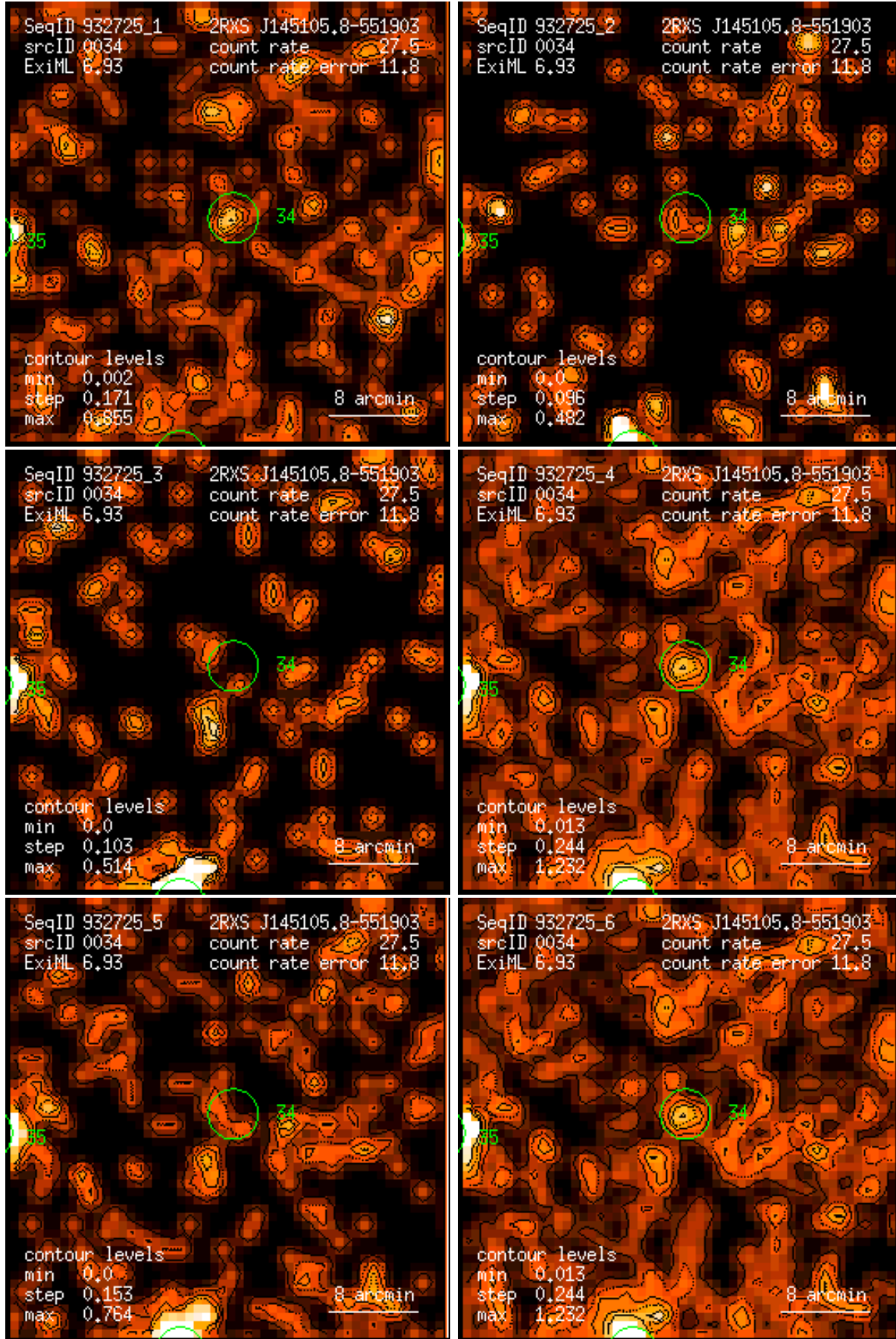
Figure 34: RASS 932725: detection 0034: band rate images, Gaussian filter: (1) PSPC channels 11 – 41, (2) 52 – 90, (3) 91 – 201, (4) 11 – 235, (5) 52 – 201, (6) 11 – 201. Broad band rates in counts/ks. Band rate contour levels in counts/ks/arcmin 2 .
