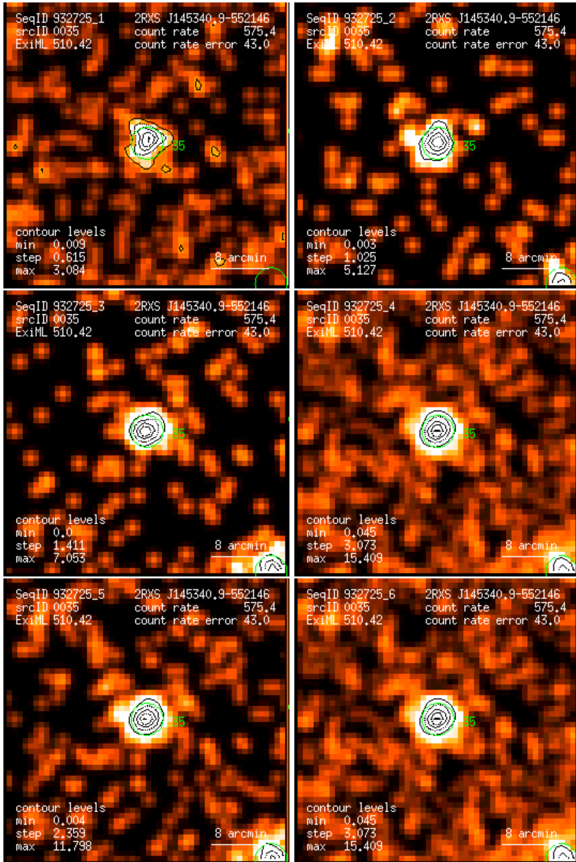
Figure 35: RASS 932725: detection 0035: band rate images, Gaussian filter: (1) PSPC channels 11 – 41, (2) 52 – 90, (3) 91 – 201, (4) 11 – 235, (5) 52 – 201, (6) 11 – 201. Broad band rates in counts/ks. Band rate contour levels in counts/ks/arcmin 2 .
