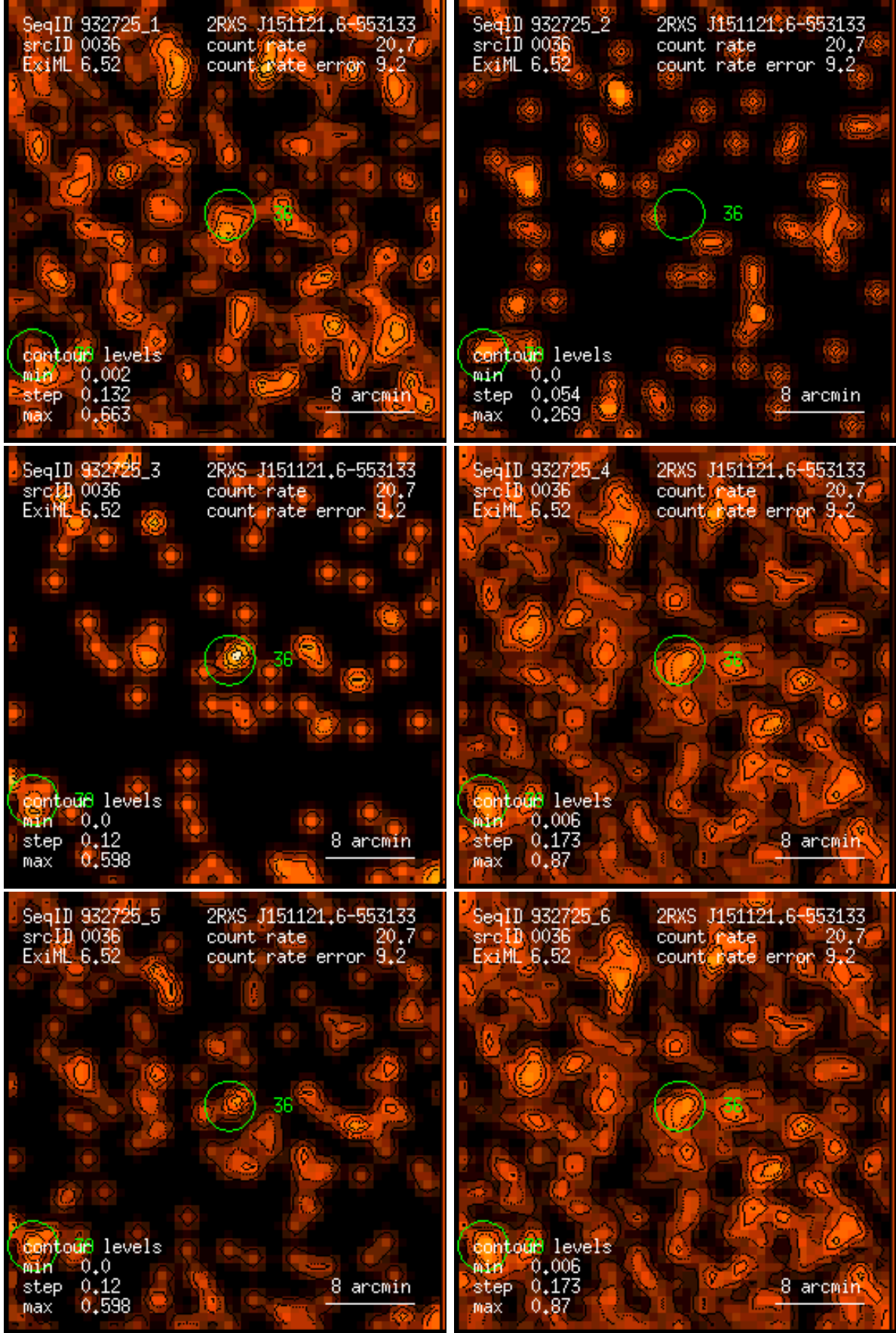
Figure 36: RASS 932725: detection 0036: band rate images, Gaussian filter: (1) PSPC channels 11 – 41, (2) 52 – 90, (3) 91 – 201, (4) 11 – 235, (5) 52 – 201, (6) 11 – 201. Broad band rates in counts/ks. Band rate contour levels in counts/ks/arcmin 2 .
