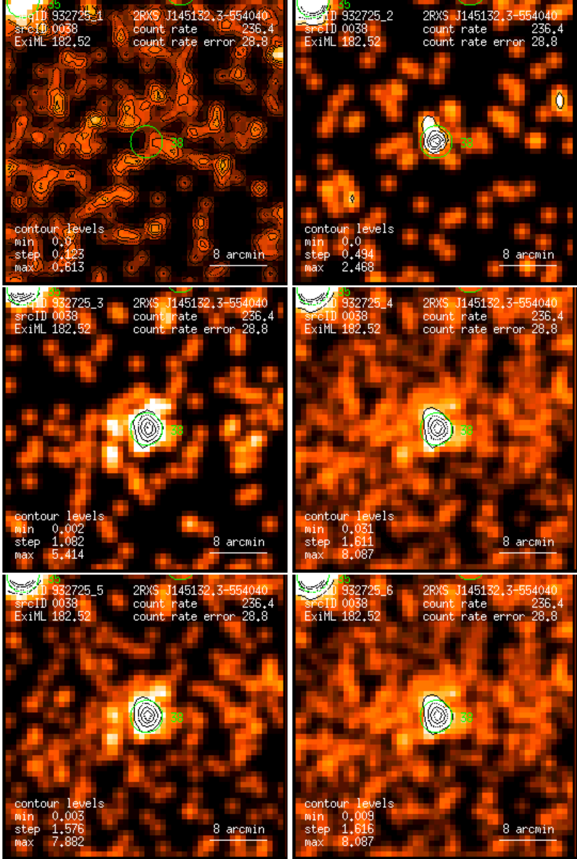
Figure 38: RASS 932725: detection 0038: band rate images, Gaussian filter: (1) PSPC channels 11 – 41, (2) 52 – 90, (3) 91 – 201, (4) 11 – 235, (5) 52 – 201, (6) 11 – 201. Broad band rates in counts/ks. Band rate contour levels in counts/ks/arcmin 2 .
