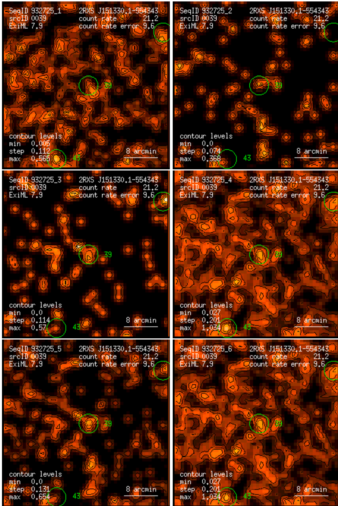
Figure 39: RASS 932725: detection 0039: band rate images, Gaussian filter: (1) PSPC channels 11 – 41, (2) 52 – 90, (3) 91 – 201, (4) 11 – 235, (5) 52 – 201, (6) 11 – 201. Broad band rates in counts/ks. Band rate contour levels in counts/ks/arcmin 2 .
