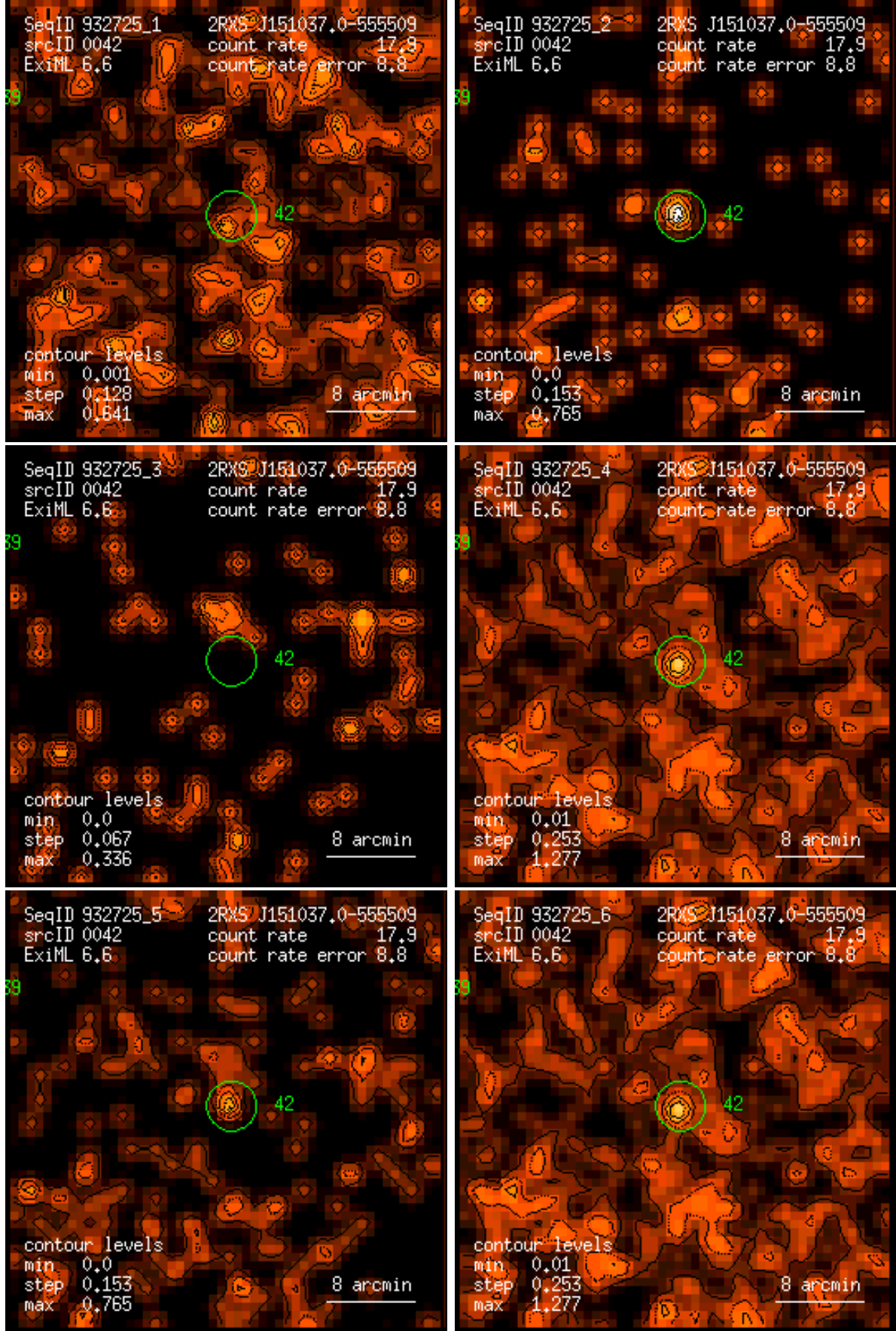
Figure 42: RASS 932725: detection 0042: band rate images, Gaussian filter: (1) PSPC channels 11 – 41, (2) 52 – 90, (3) 91 – 201, (4) 11 – 235, (5) 52 – 201, (6) 11 – 201. Broad band rates in counts/ks. Band rate contour levels in counts/ks/arcmin 2 .
