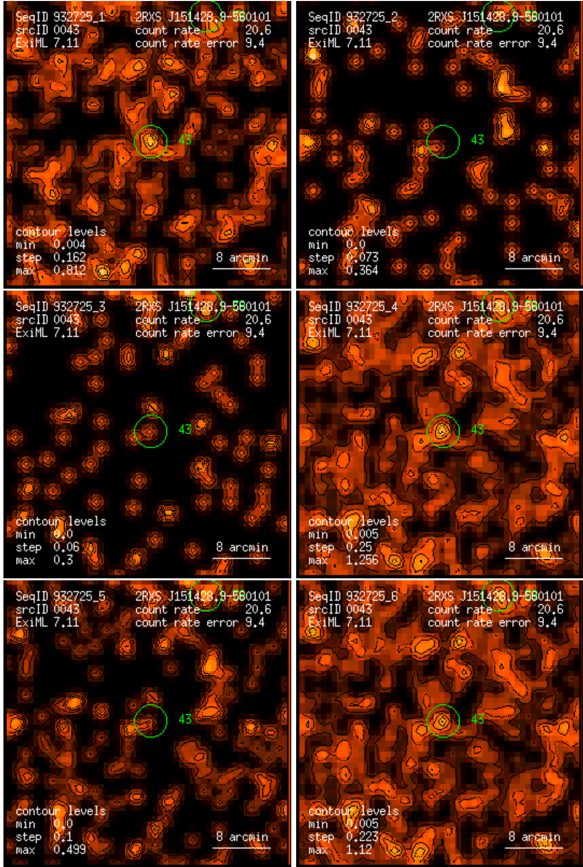
Figure 43: RASS 932725: detection 0043: band rate images, Gaussian filter: (1) PSPC channels 11 – 41, (2) 52 – 90, (3) 91 – 201, (4) 11 – 235, (5) 52 – 201, (6) 11 – 201. Broad band rates in counts/ks. Band rate contour levels in counts/ks/arcmin 2 .
