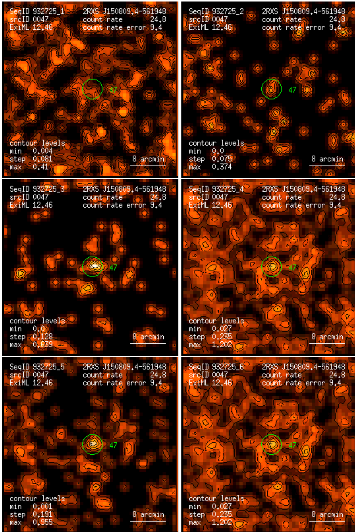
Figure 47: RASS 932725: detection 0047: band rate images, Gaussian filter: (1) PSPC channels 11 – 41, (2) 52 – 90, (3) 91 – 201, (4) 11 – 235, (5) 52 – 201, (6) 11 – 201. Broad band rates in counts/ks. Band rate contour levels in counts/ks/arcmin 2 .
